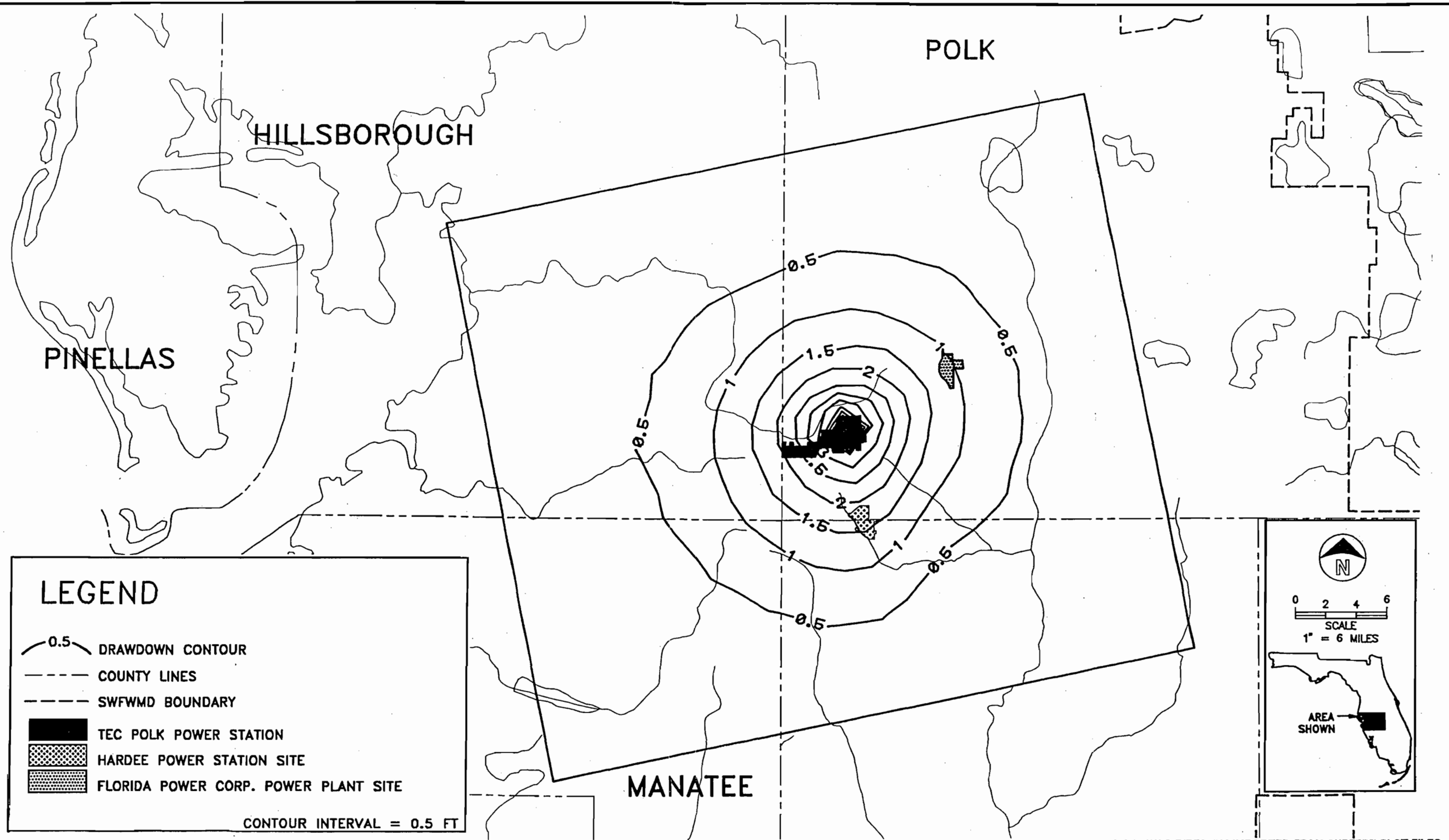
FIGURE 4.3.1-5. Drawdown in the Floridan Aquifer Transient Conditions - 45 Days (Case 1), Tampa Electric Company - Polk Power Station.
