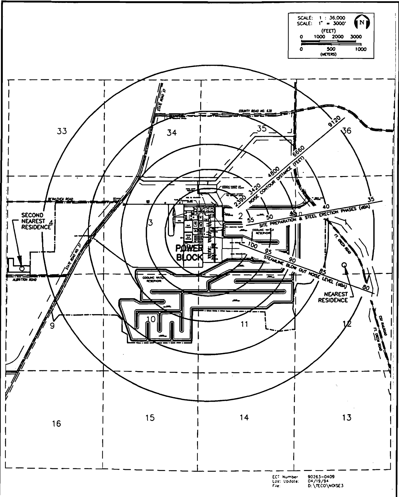
FIGURE 4.11.1-1. Composite Construction Noise-Level Contours.
