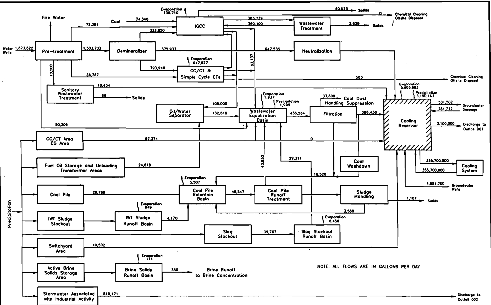
FIGURE 4.12.2-1. Water Mass Balance, Annual Average Makeup.
