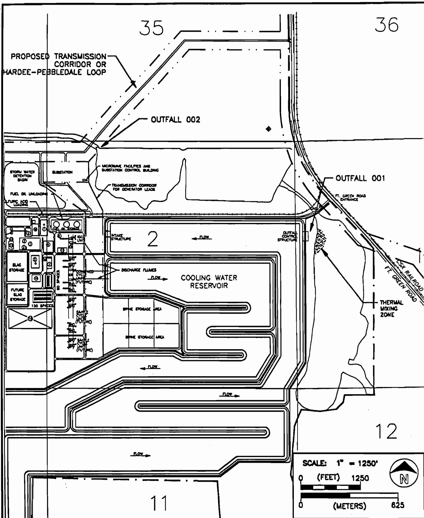
FIGURE 4.2.1-2. Thermal Mixing Zone (Full Load and Maximum Discharges).
