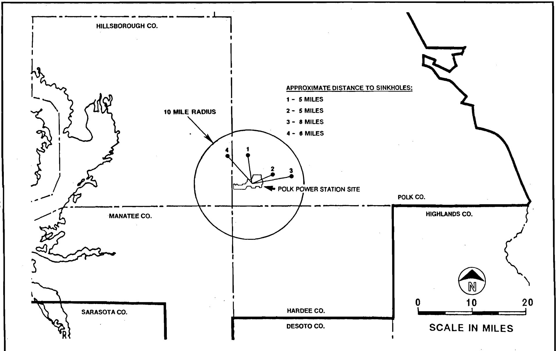
FIGURE 3.4.4-3. Sinkhole Identification Map.
