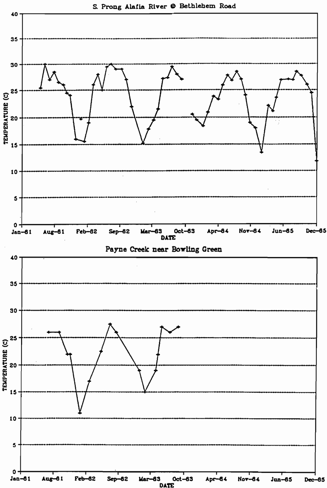
FIGURE 3.2.3-1. Historical Water Temperature Data for South Prong Alafia River and Payne Creek.
