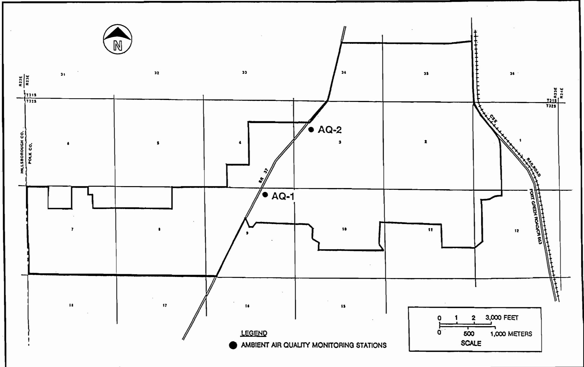
FIGURE 3.1.2-1. Ambient Air Monitoring Stations.
