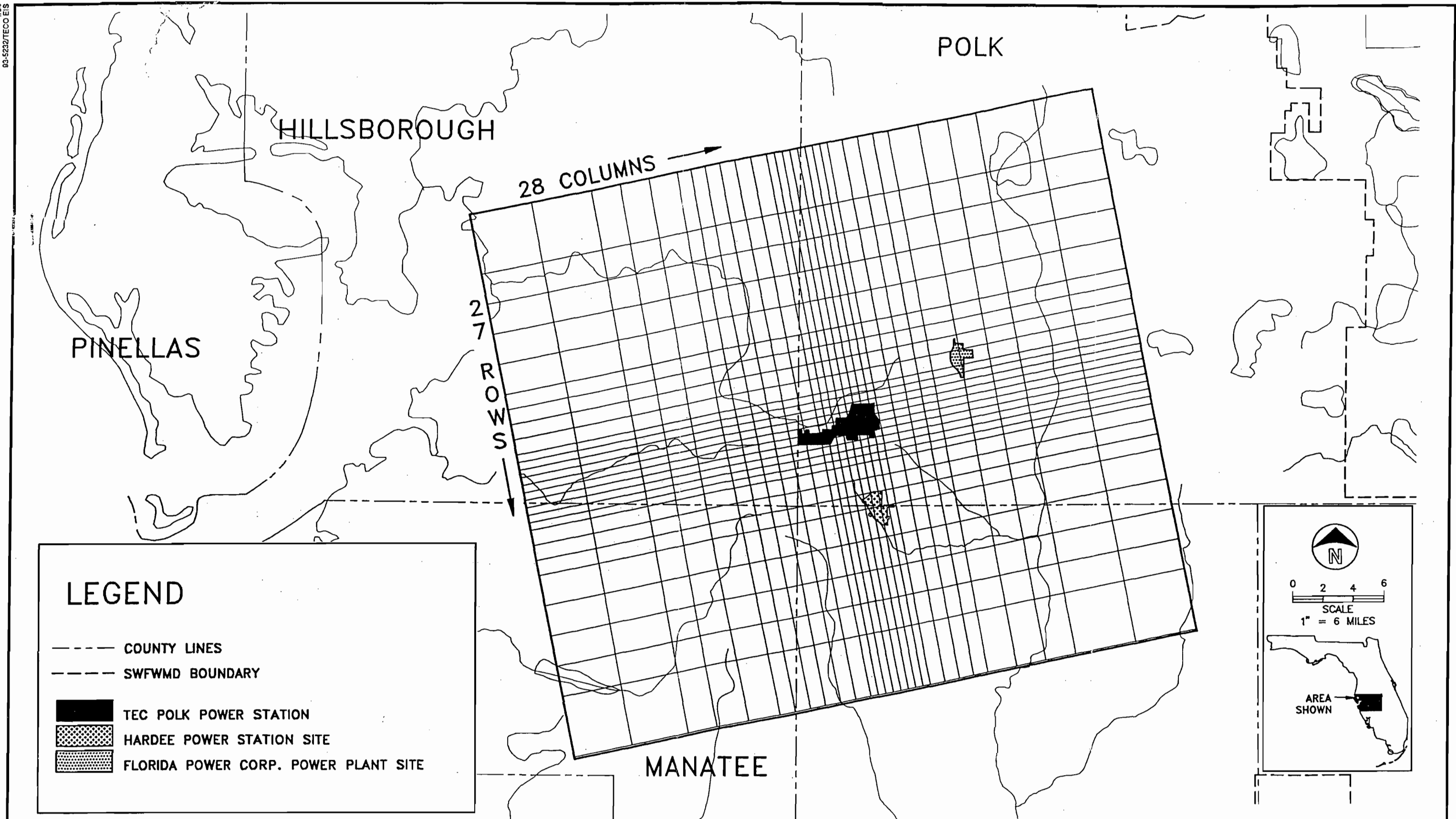
FIGURE 4.3.1-4. Floridan Aquifer Model Grid, Tampa Electric Company - Polk Power Station.
