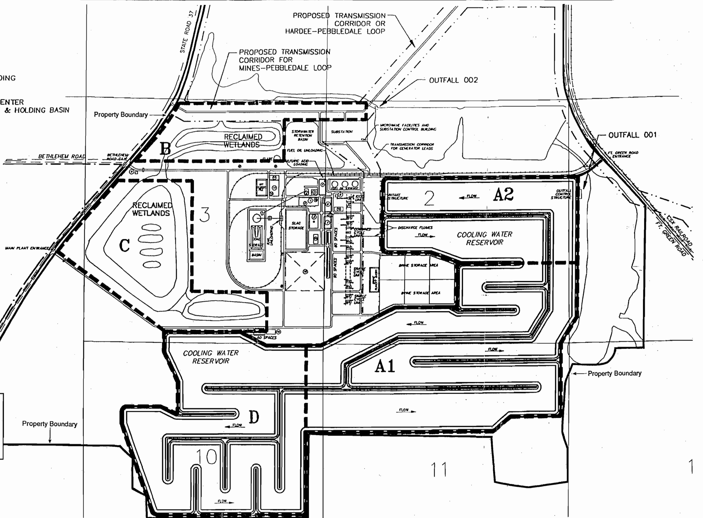
FIGURE 4.3.1-1. Dewatering Subareas for Cooling Water Reservoir and Wetland Areas.
