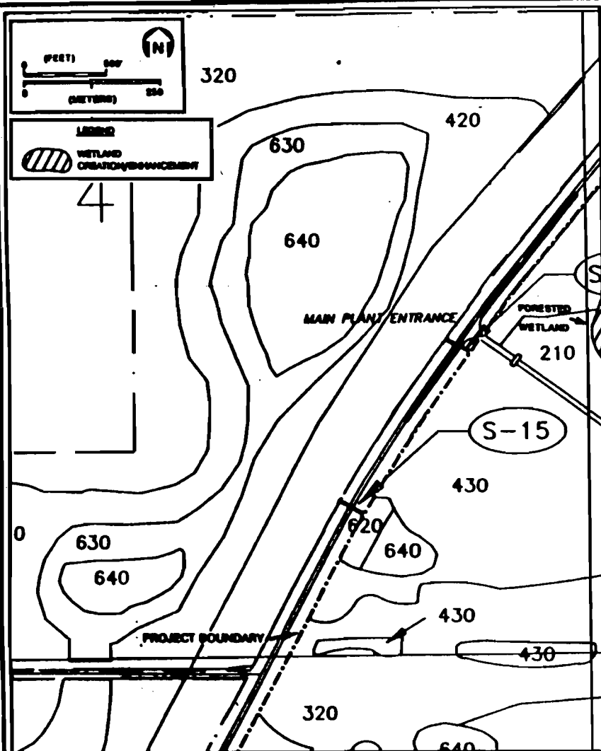
FIGURE 4. (PAGE 5 OF 13) SEE KEY POST-RECLAMATION LAND USE WITH WETLAND CREATION/ENHANCEMENT AREAS DEPICTED DREDGE AND FILL PERMIT APPLICATION Source: SCT, 1988.
