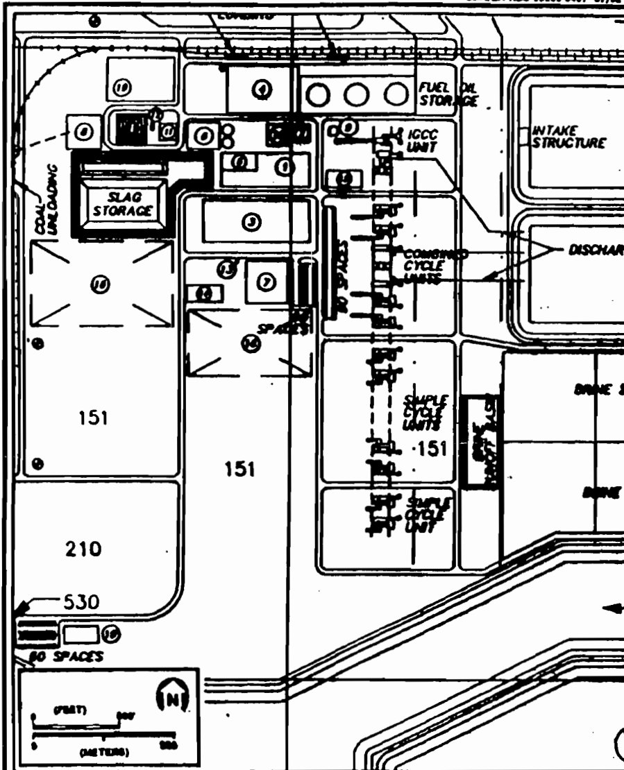
FIGURE 4. (PAGE 7 OF 13) See Key POST-RECLAMATION LAND USE WITH WETLAND CREATION/ENHANCEMENT AREAS DEPICTED DREDGE AND FILL PERMIT APPLICATION Source: DEC, 1992.
