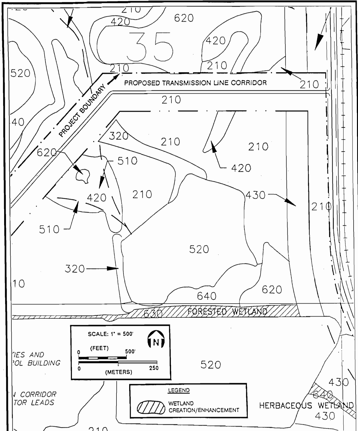
FIGURE 5. (PAGE 3 OF 13) POST-RECLAMATION LAND USE WITH WETLAND CREATION/ENHANCEMENT AREAS DEPICTED DREDGE AND FILL PERMIT APPLICATION
