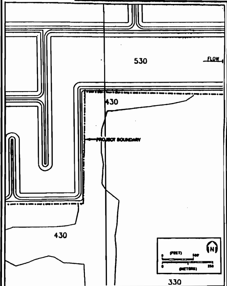
FIGURE 4 (PAGE 12 OF 13) See Key POST-RECLAMATION LAND USE WITH WETLAND CREATION/ENHANCEMENT AREAS DEPICTED DREDGE AND FILL PERMIT APPLICATION Revised 08/92, 10/92.
