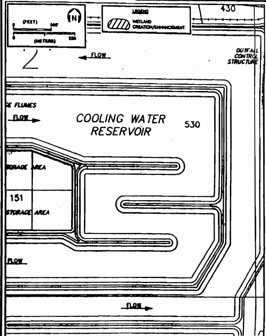
FIGURE 4. (PAGE 8 OF 13) See Key POST-RECLAMATION LAND USE WITH WETLAND CREATION/ENHANCEMENT AREAS DEPICTED DREDGE AND FILL PERMIT APPLICATION Source: DEC, 1992.
