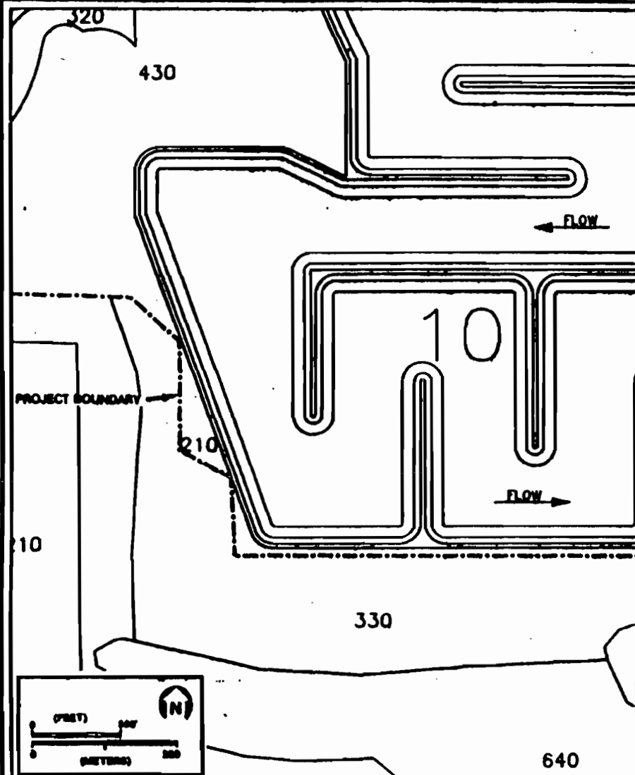
FIGURE 4 (PAGE 11 OF 13) See Key POST-RECLAMATION LAND USE WITH WETLAND CREATION/ENHANCEMENT AREAS DEPICTED DREDGE AND FILL PERMIT APPLICATION Revised 08/92, 10/92.
