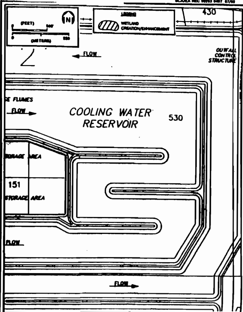
FIGURE 4. (PAGE 8 OF 13) SEE KEY POST-RECLAMATION LAND USE WITH WETLAND CREATION/ENHANCEMENT AREAS DEPICTED DREDGE AND FILL PERMIT APPLICATION
