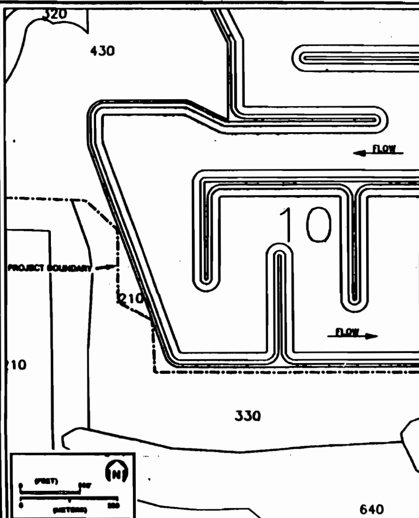
FIGURE 4. (PAGE 11 OF 13) See Key POST-RECLAMATION LAND USE WITH WETLAND CREATION/ENHANCEMENT AREAS DEPICTED DREDGE AND FILL PERMIT APPLICATION Revised: 09/09/92
