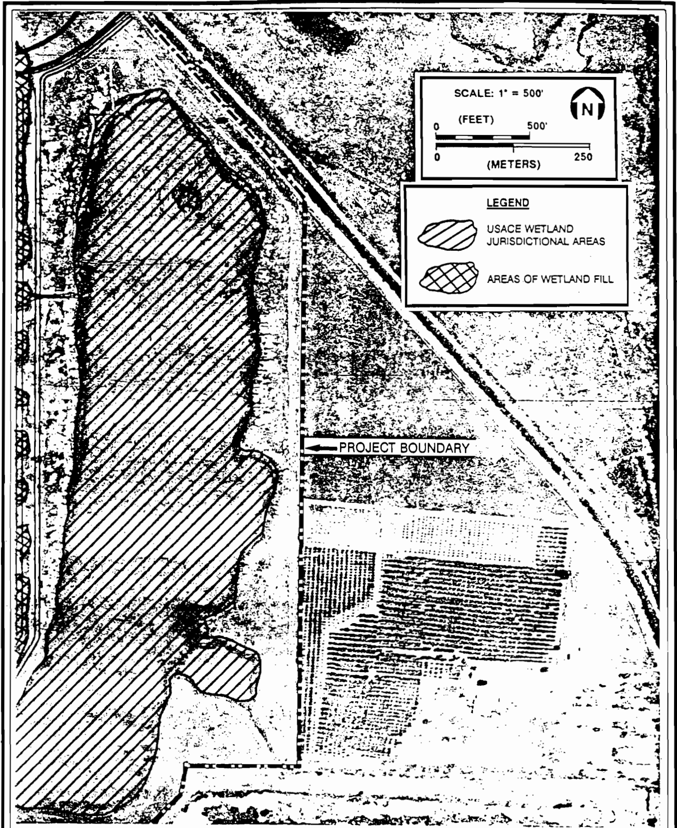
FIGURE 3. AERIAL PHOTOGRAPHY WITH USACE WETLAND DELINEATIONS (PAGE 9 OF 13) DREDGE AND FILL PERMIT APPLICATION Sources: I.F. Rocks & Assoc. Inc.; ECT, 1992.
