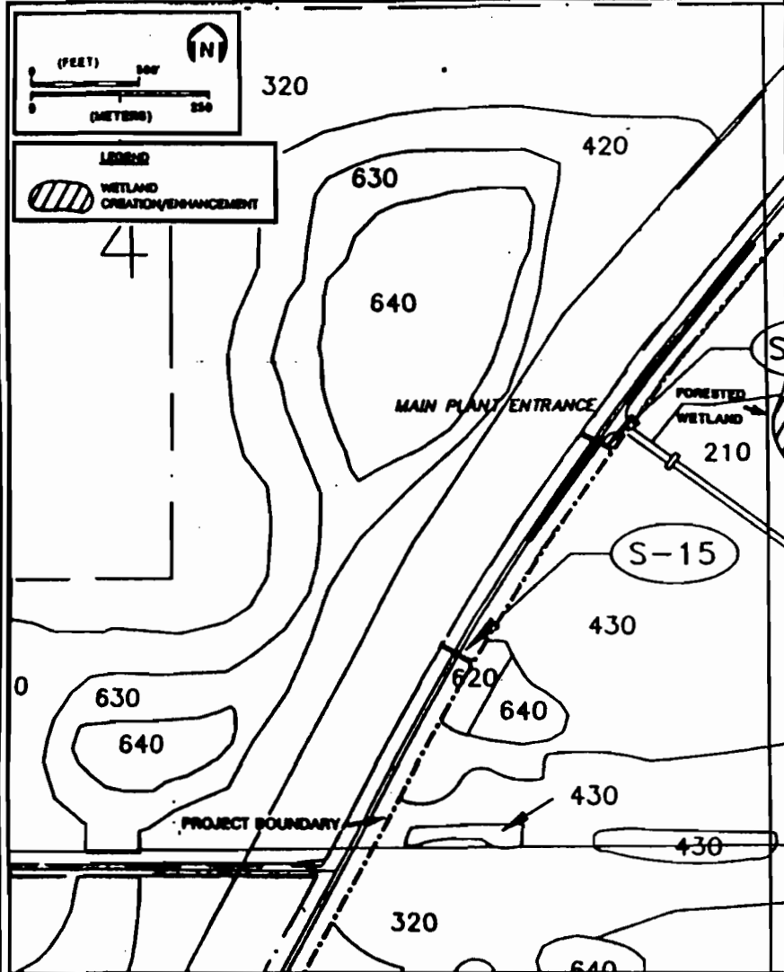
FIGURE 4 (PAGE 5 OF 13) SEE KEY POST-RECLAMATION LAND USE WITH WETLAND CREATION/ENHANCEMENT AREAS DEPICTED DREDGE AND FILL PERMIT APPLICATION Source: BCT, 1988.
