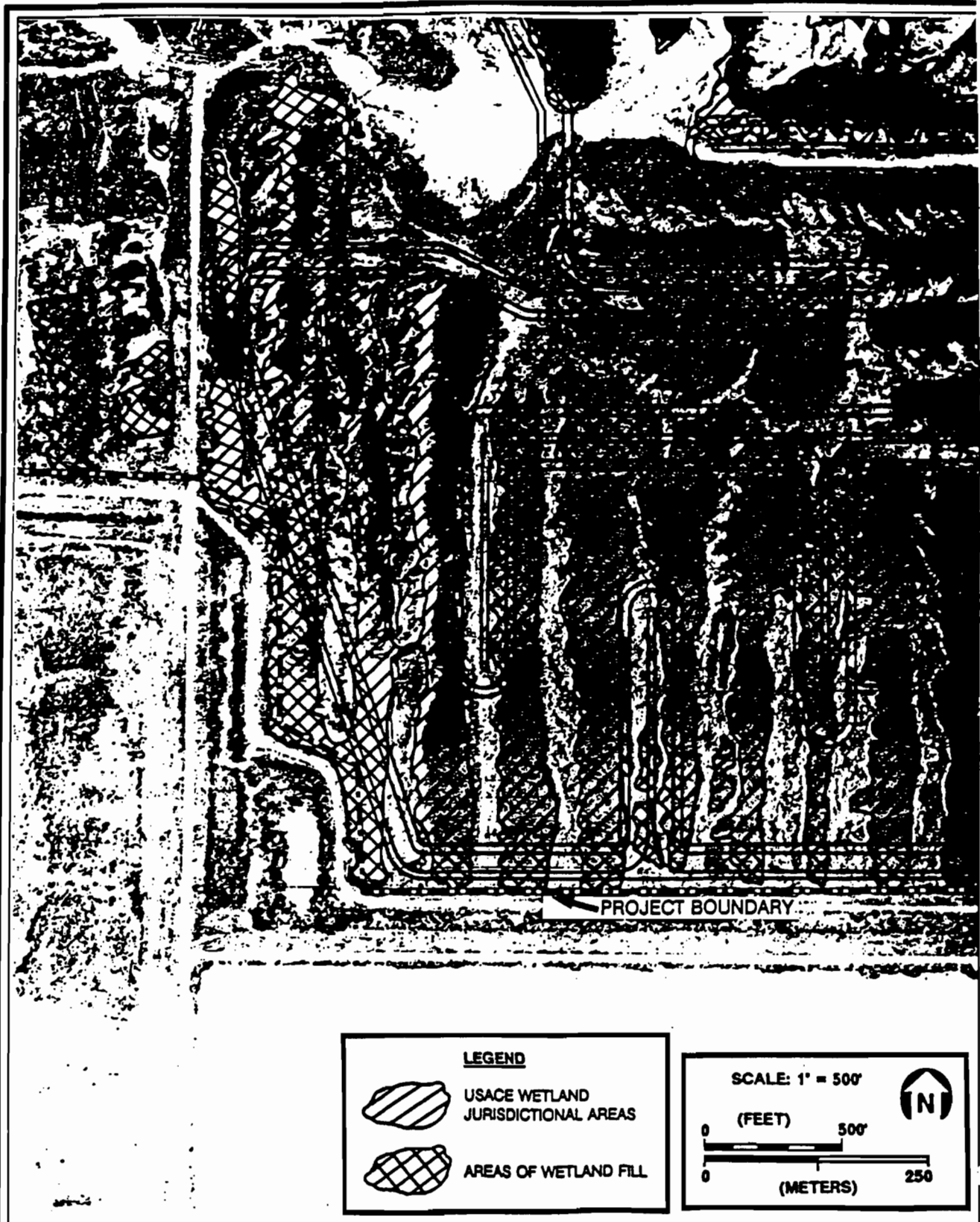
FIGURE 3. AERIAL PHOTOGRAPHY WITH USACE WETLAND DELINEATIONS (PAGE 11 OF 13) DREDGE AND FILL PERMIT APPLICATION Sources: L.F. Rooks & Assoc. Inc.; ECT, 1992.
