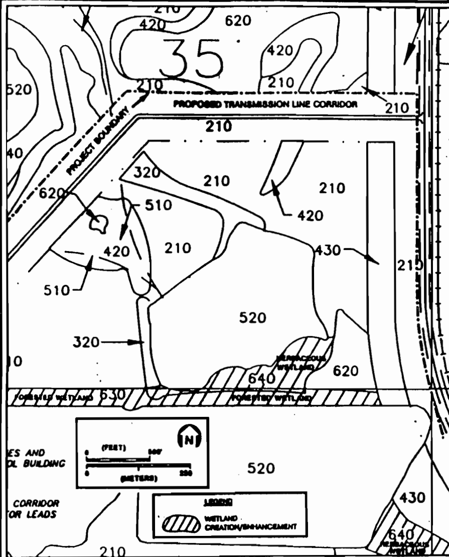
FIGURE 4 (PAGE 3 OF 13) SEE KEY POST-RECLAMATION LAND USE WITH WETLAND CREATION/ENHANCEMENT AREAS DEPICTED DREDGE AND FILL PERMIT APPLICATION Source: SCT, 1992.
