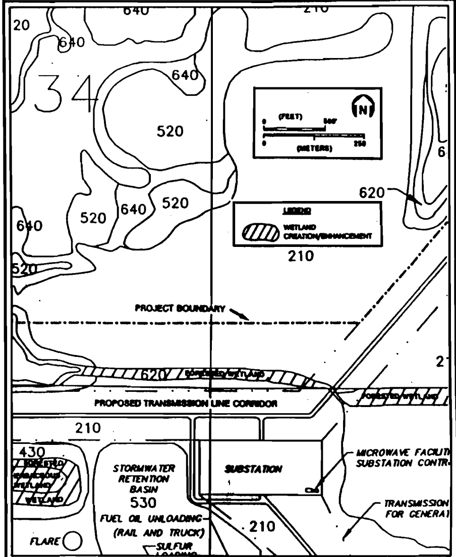
FIGURE 4. (PAGE 2 OF 13) - SEE KEY POST-RECLAMATION LAND USE WITH WETLAND CREATION/ENHANCEMENT AREAS DEPICTED DREDGE AND FILL PERMIT APPLICATION Sources: BCT, 1988.
