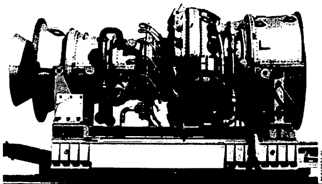
Figure 3. A GE 7FA on a half-shell Figure 4. Preassembled GE 7FA ready for shipping
