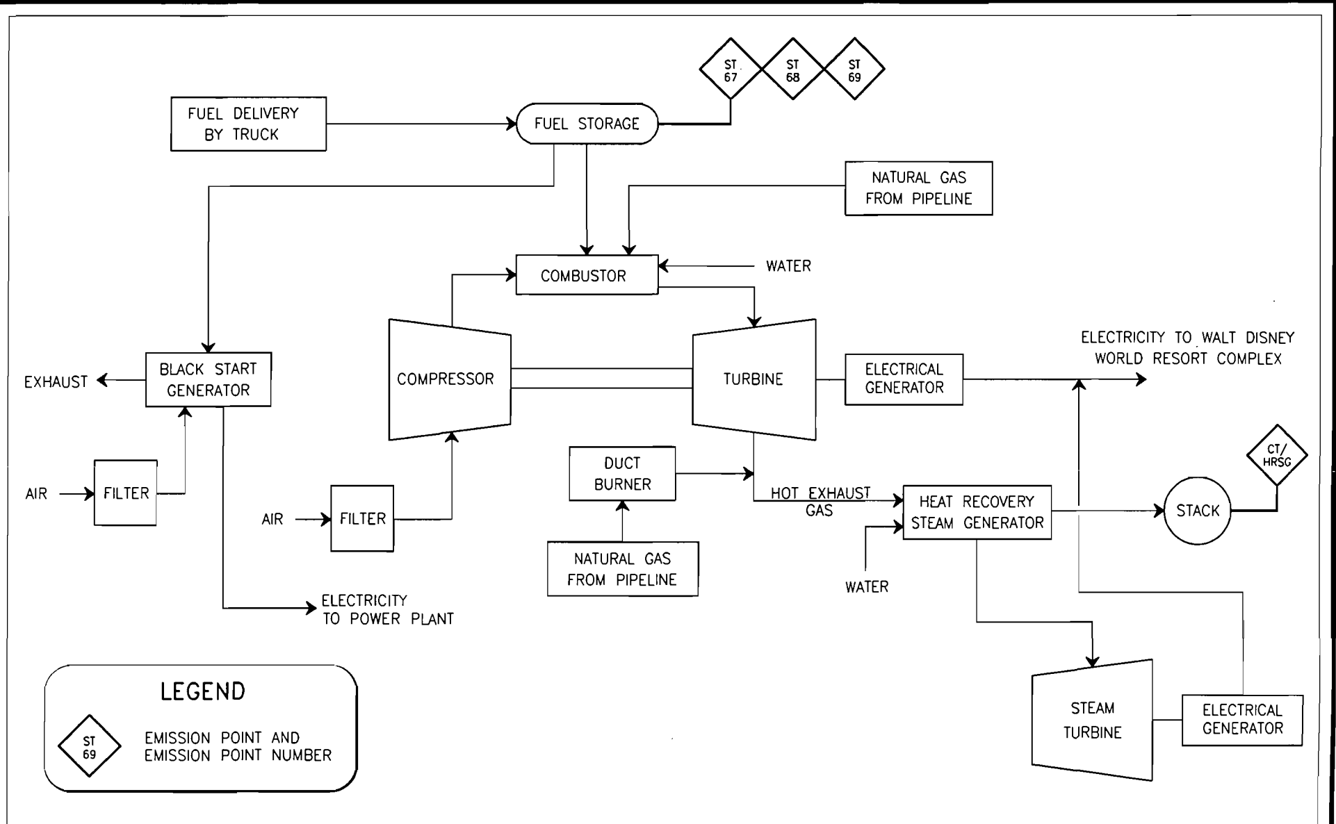
FIGURE II.D.3.1. WALT DISNEY WORLD RESORT COMPLEX: PROCESS SCHEMATIC DIAGRAM NORTH SERVICE AREA COMBUSTION TURBINE Source: ECT, 1996.
