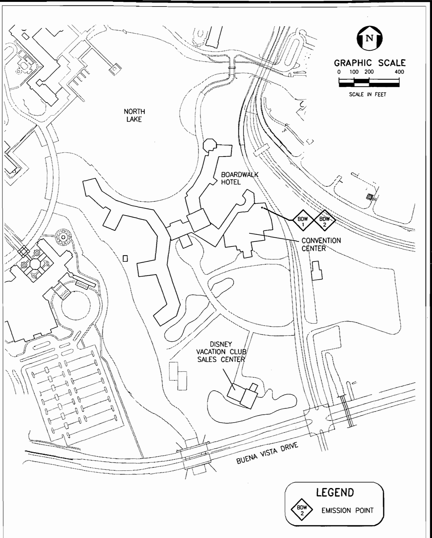
FIGURE II.D.2.6. WALT DISNEY WORLD RESORT COMPLEX EMISSION SOURCE LOCATION DISNEY'S BOARDWALK RESORT
