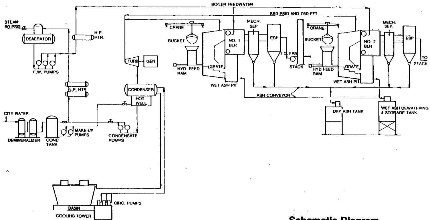
Schematic Diagram Electrical Generation
