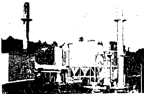
FIG. 4 FRAMINGHAM INSTALLATION
