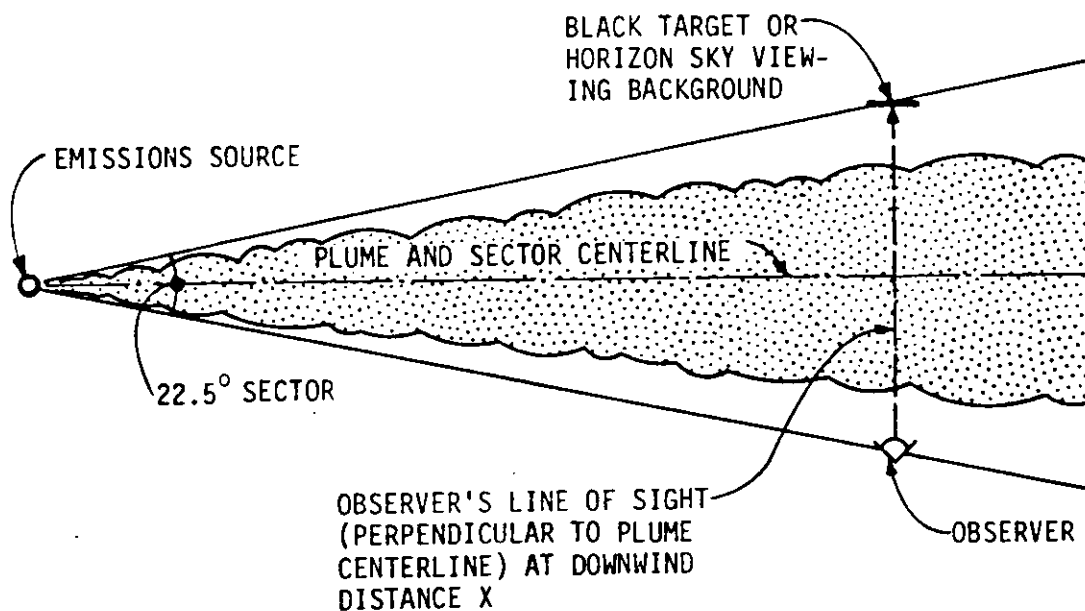
Geometry of plume, observer, and line of sight used in level-1 visibility screening analysis.
