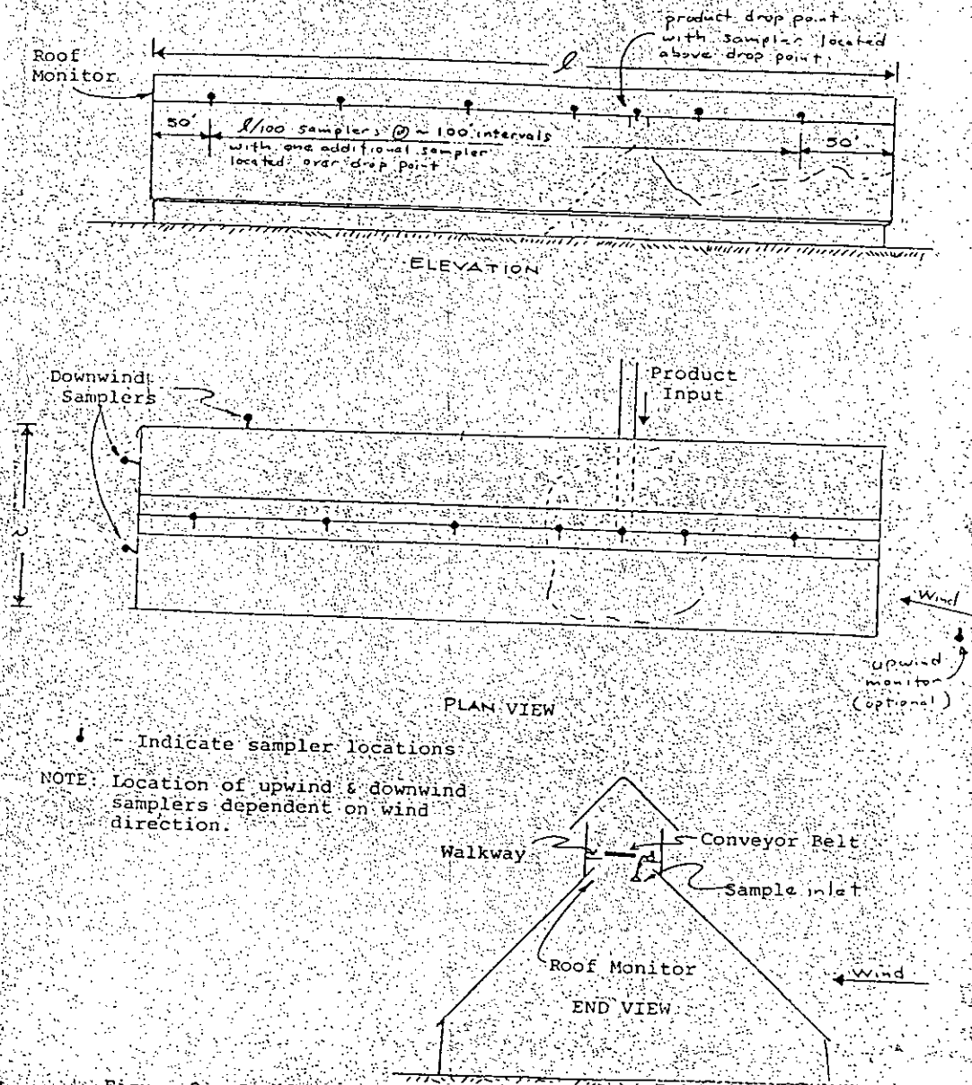
Figure 2. Sampler Locations
