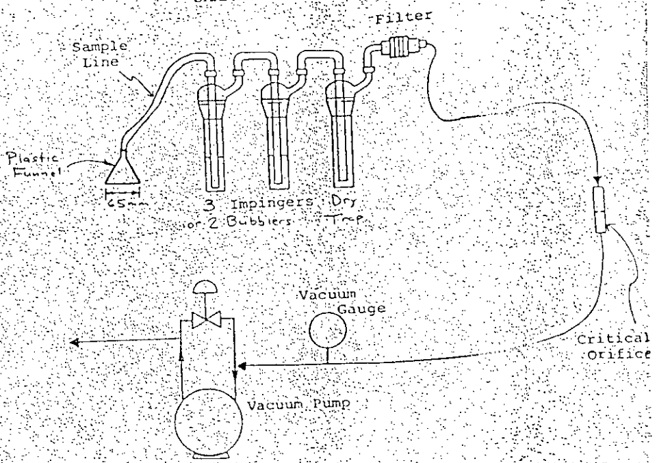
Figure 1 SAMPLING TRAIN
