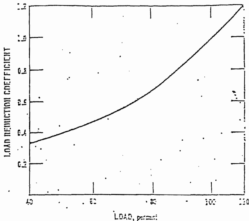
Figure 1.4-1. Load reduction coefficient as a function of boiler load. (Used to determine \text{NO}_x reductions at reduced loads in large boilers.)
