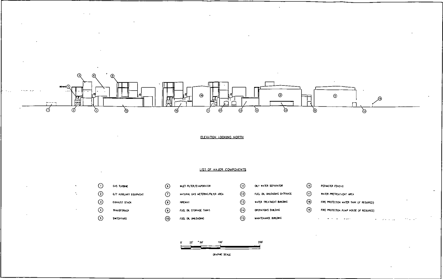
FIGURE 2-6. SITE ELEVATION LOOKING NORTH FOR THE PROPOSED OLEANDER POWER PLANT
