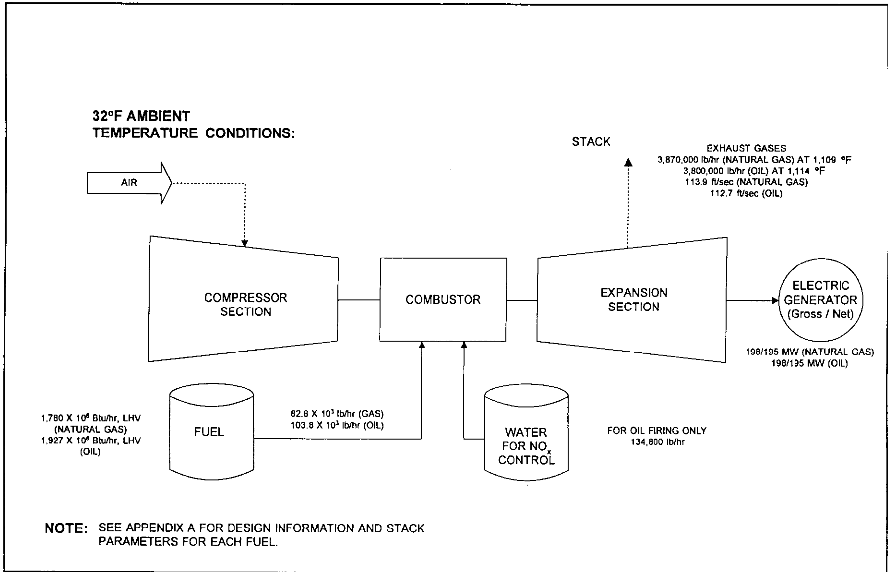
Figure 2-4 Simplified Flow Diagram of Proposed "F" Class Combustion Turbine Baseload, Winter Design Conditions Proposed Oleander Power Project
