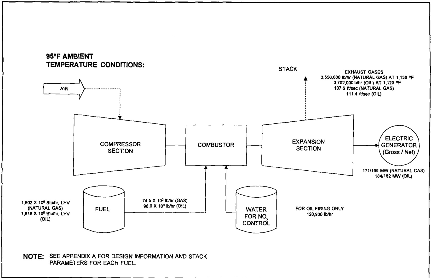
Figure 2-2 Simplified Flow Diagram of Proposed "F" Class Combustion Turbine Baseload, Summer Design Conditions Proposed Oleander Power Project
