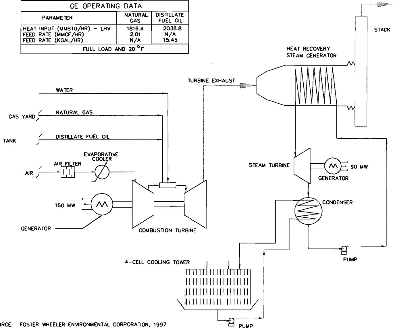
SIMPLIFIED PROCESS FLOW DIAGRAM PURDOM UNIT 8 PROJECT - ST MARKS, FLORIDA REVISED: NOVEMBER 9, 2001
