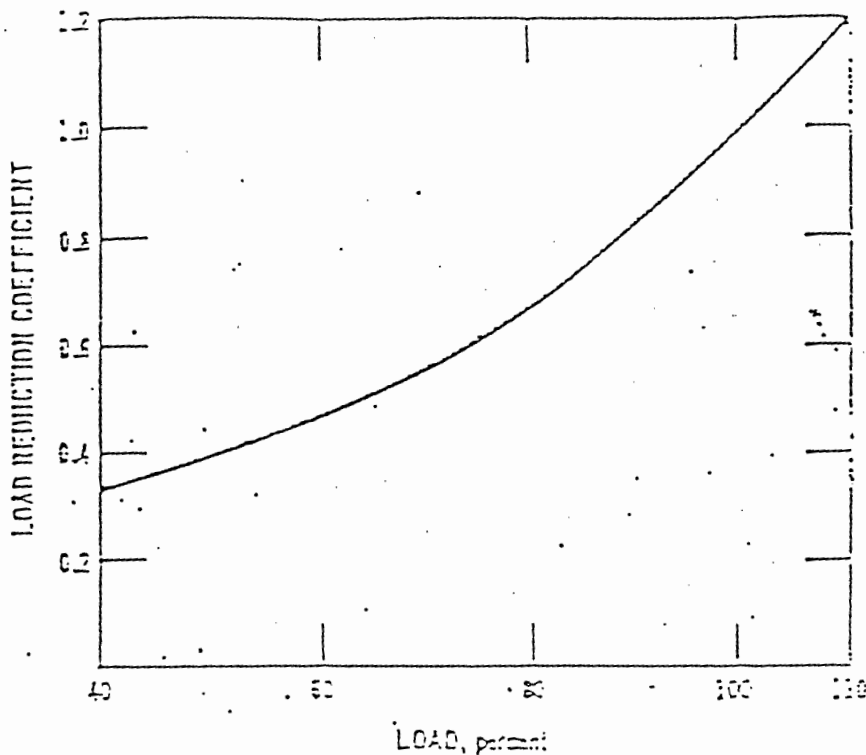
Figure 1.4-1. Load reduction coefficient as a function of boiler load. (Used to determine \text{NO}_2 reductions at reduced loads in large boilers.)
