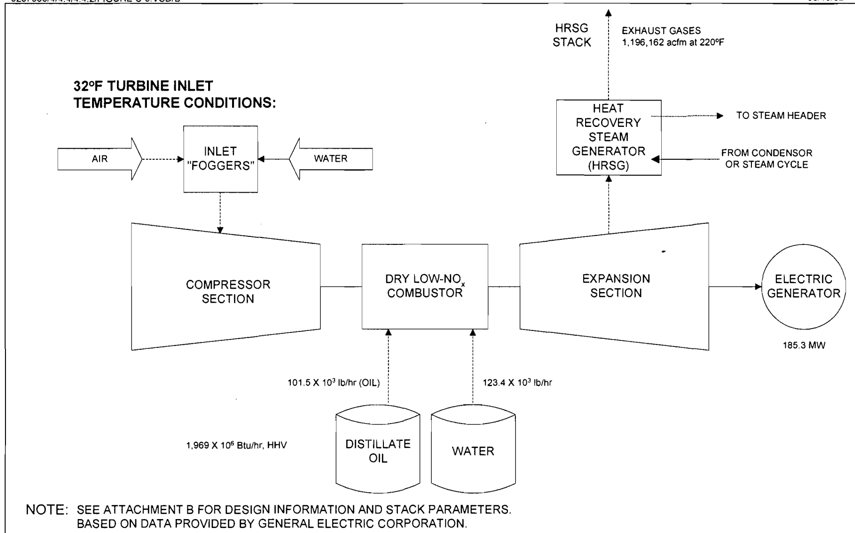
Figure C-3B Simplified Flow Diagram of Units 5A-5D Distillate Oil Firing Sanford Repowering Project
