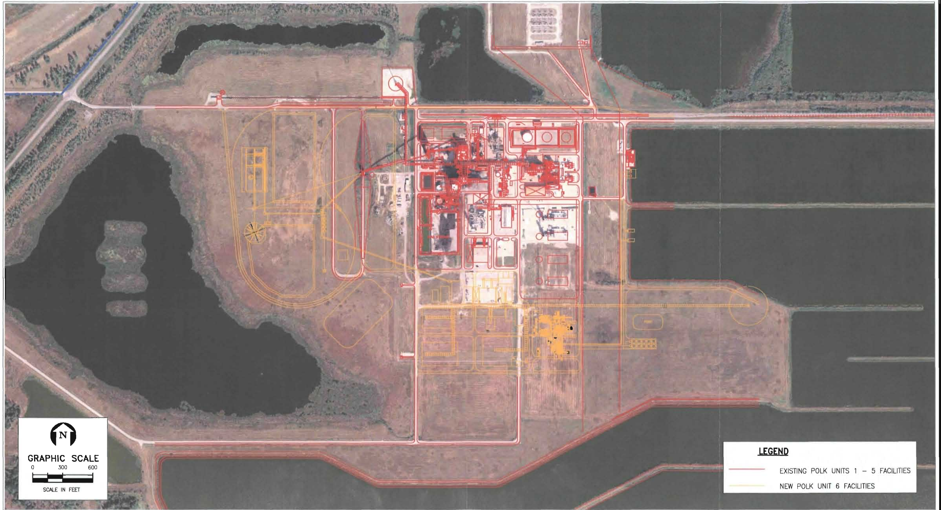
FIGURE 2-3. DETAILED LAYOUT OF FACILITIES ON AERIAL PHOTOGRAPH
