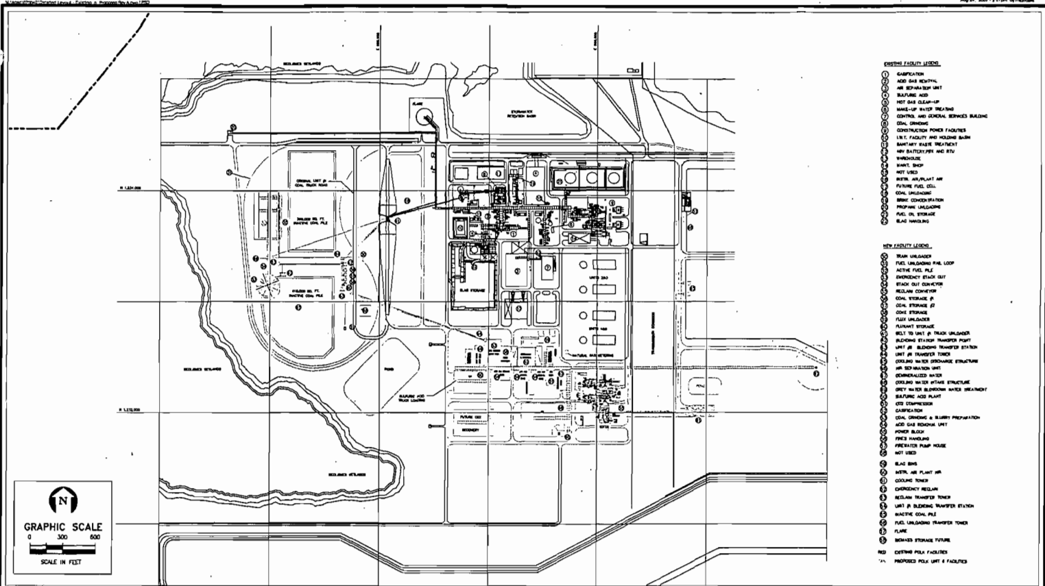
FIGURE 2-2. DETAILED LAYOUT OF EXISTING AND PROPOSED POLK UNIT 6 FACILITIES
