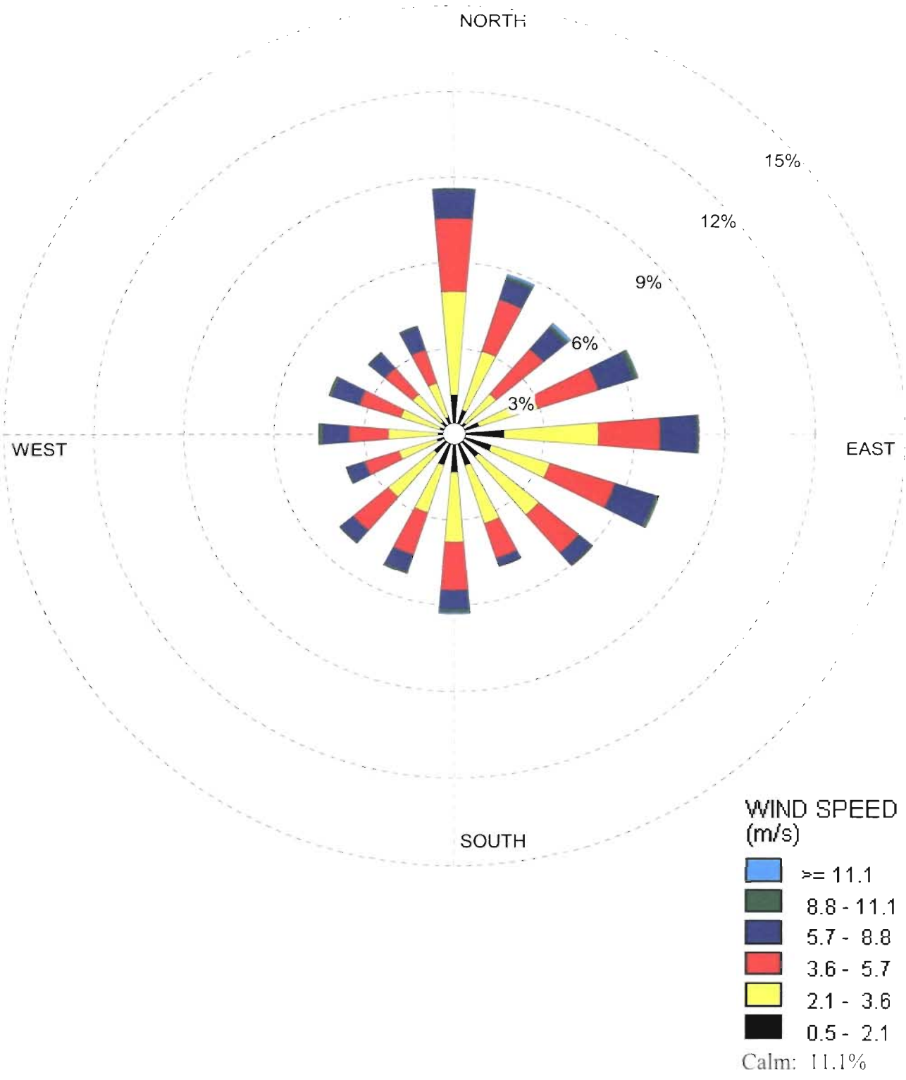
FIGURE 6-7. WIND ROSE FOR ORLANDO INTL AIRPORT (2003-2004)
