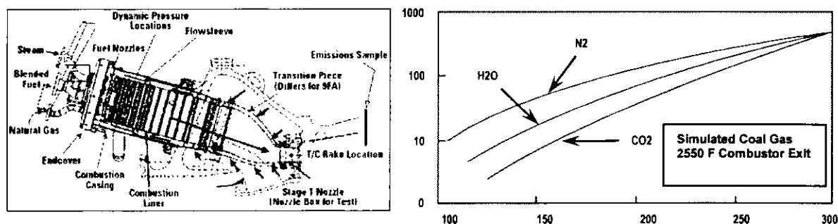
Figure 12. MNQC and Full Load NO_x (ppmvd) Performance vs. Heating Value (Btu/scf)
