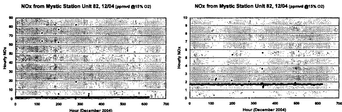
Figure 15. Hourly NO x Data from Site Mystic Station, Massachusetts. December 2004
