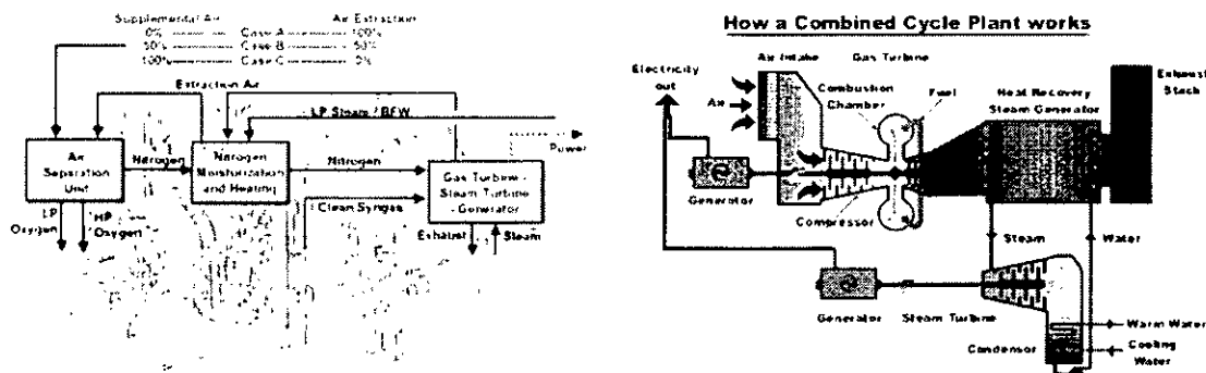
Figure 10. Integrations of CT with Gasifier Oxidant Supply and in Combined Cycle
