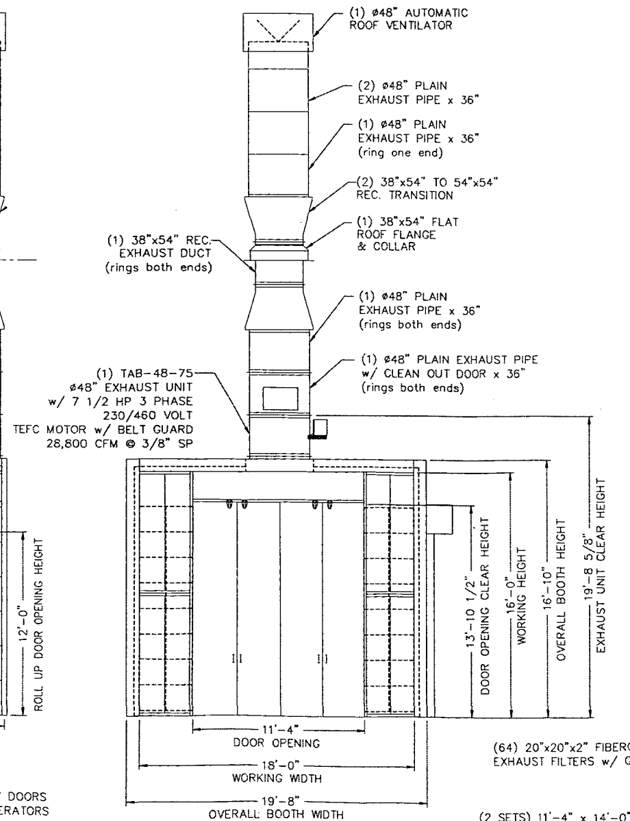
EXHAUST CHAMBER ELEVATION
