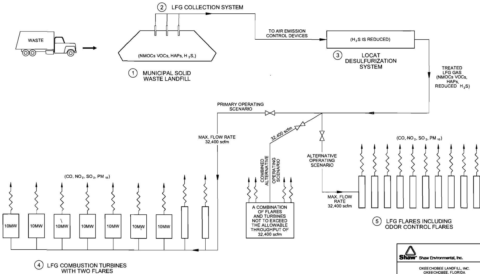
FIGURE 2 FACILITY ID 0930104 PROCESS FLOW DIAGRAM AIR CONSTRUCTION PERMIT APPLICATION 1270-2
