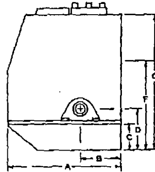
MODELS — 3623, 3633, 4326, 4340, 5348 & 6360
