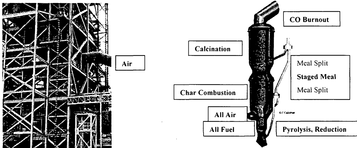
Figure 7. Titan Florida Pennsuco Cement Plant Calciner, Diagram of SCC Strategy
