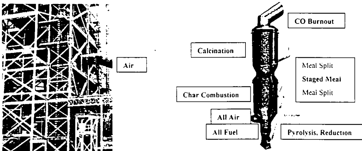
Figure 7. Titan Florida Pennsco Cement Plant Calciner, Diagram of SCC Strategy
