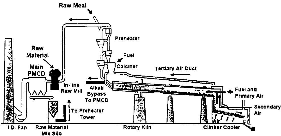
Figure 6. Process Diagram of Dry Process Preheater/Calciner Pyroprocessing System
