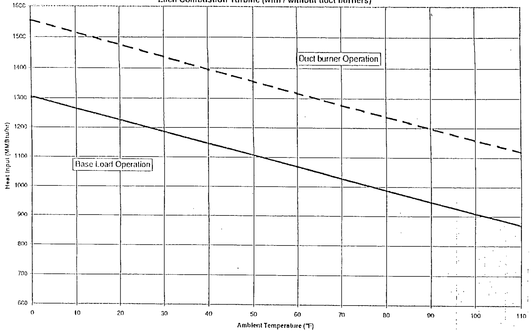
Putnam Plant Unit 1 or 2 Heat Input Variation With Ambient Temperature Each Combustion Turbine (with / without duct burners)
