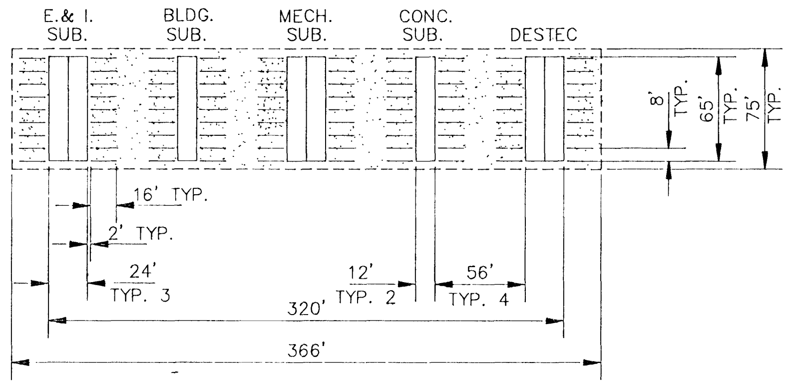
CONSTRUCTION TRAILER AREA DETAIL (NOTE 5)
