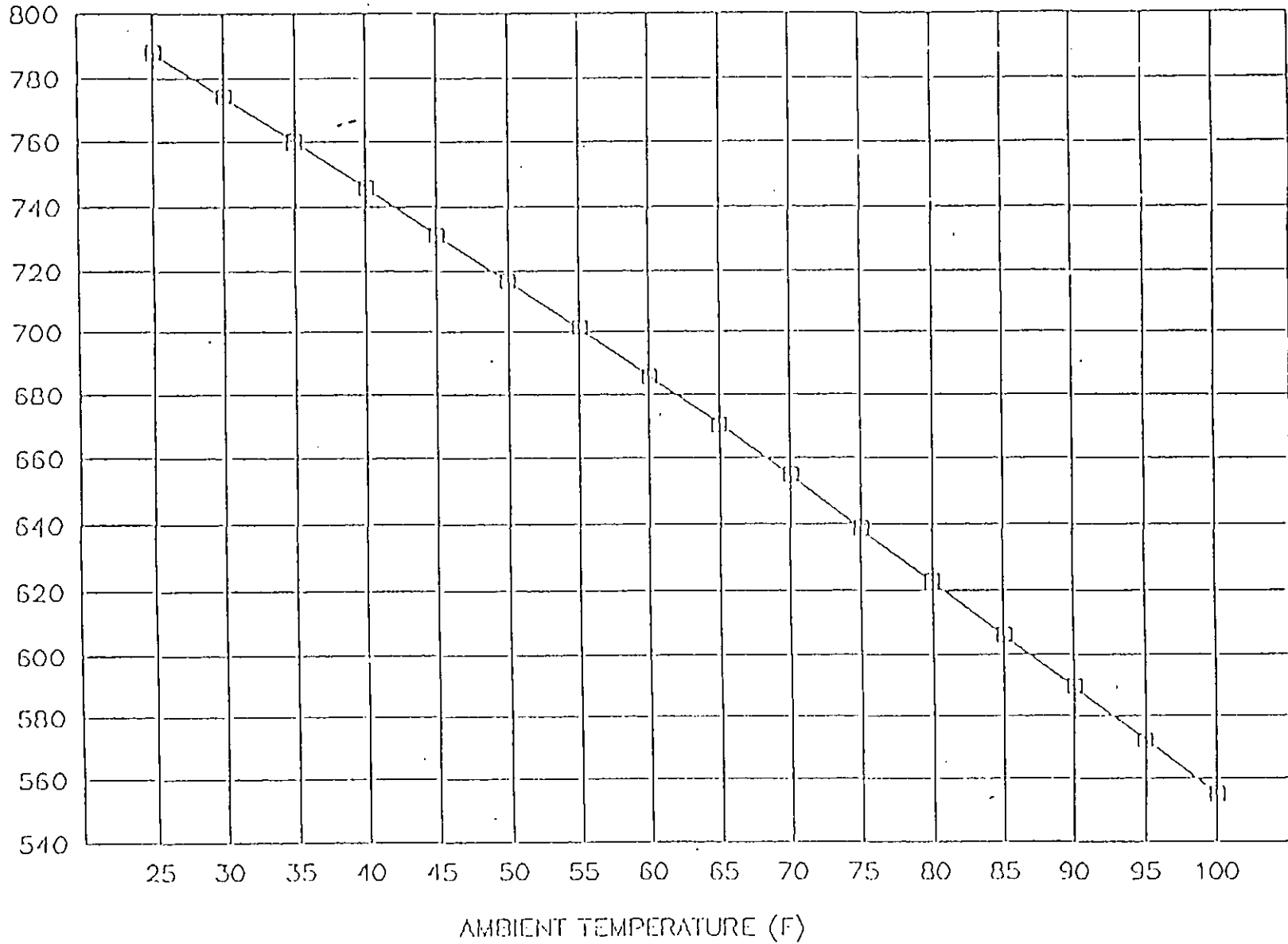
FUEL HEAT INPUT vs AMBIENT TEMPERATURE
