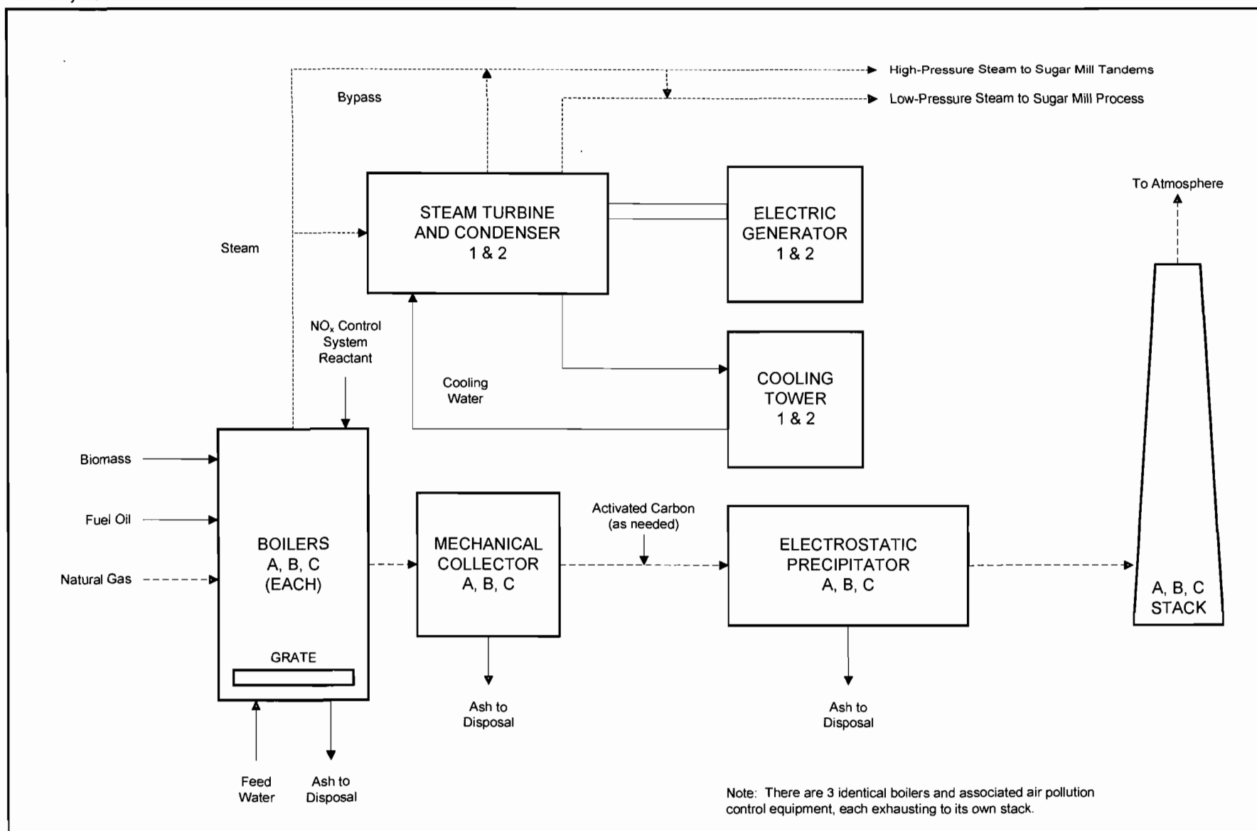
Figure 2-5 Simplified Flow Diagram – Existing Boilers New Hope Power Company, Okeelanta Cogeneration Facility South Bay, FL
