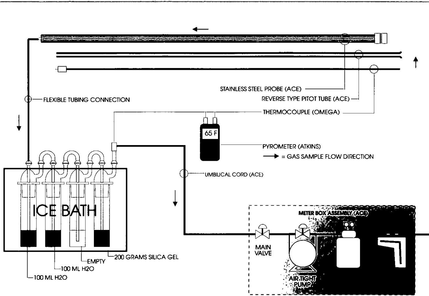
FIGURE 3. EPA METHOD 1-4 SAMPLING SCHEMATIC (DETERMINATION OF FLOW RATE FROM STATIONARY SOURCES)
