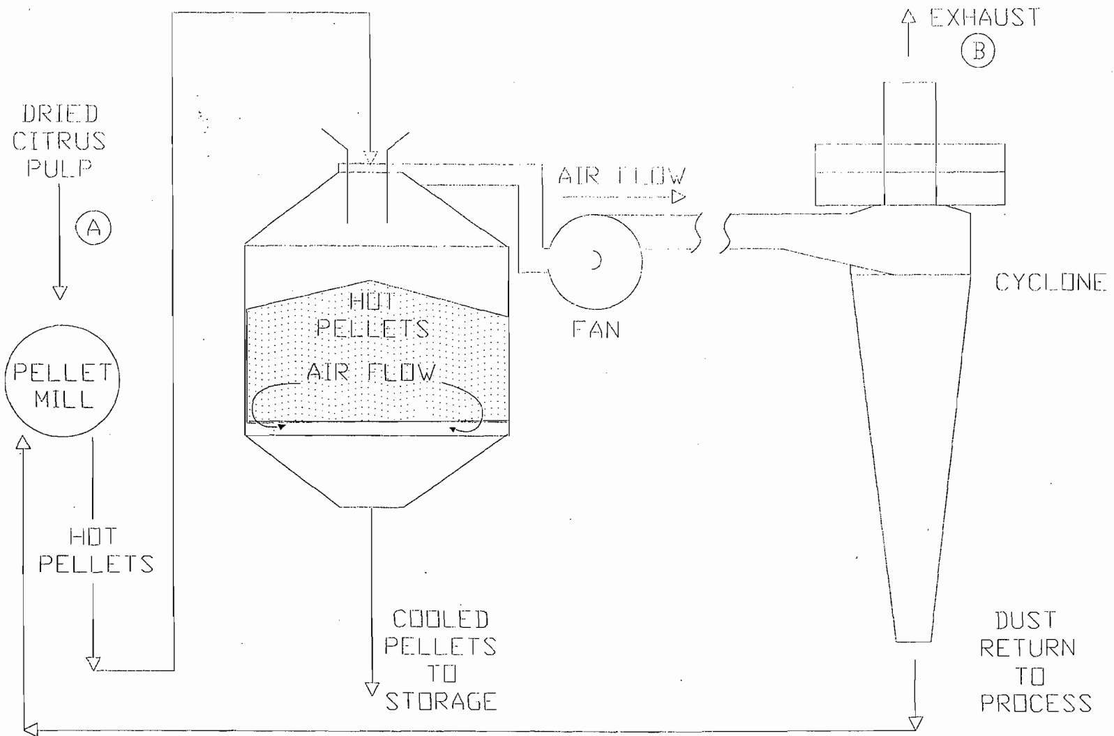
FLOW DIAGRAM
