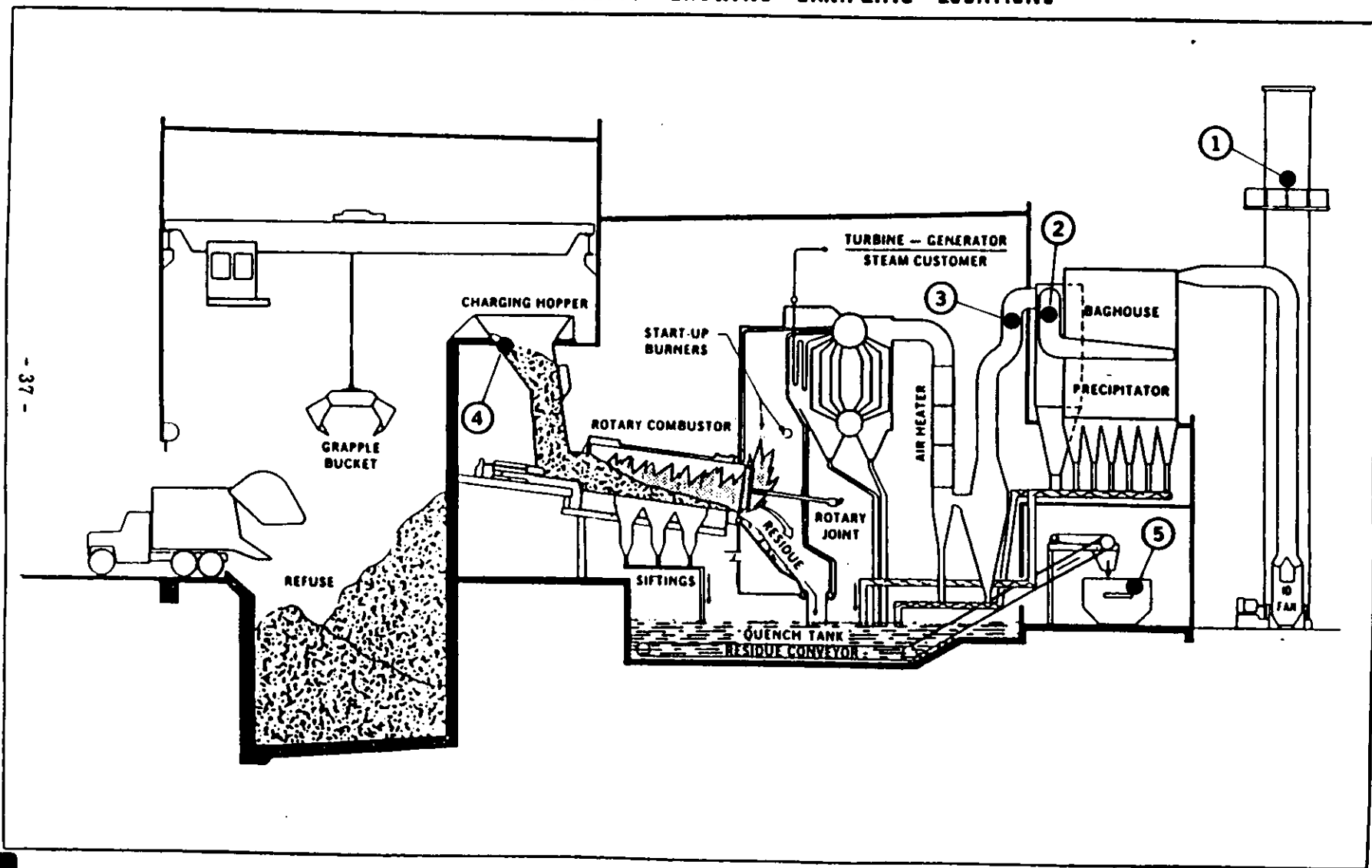
FIGURE 4-1 CROSS-SECTION OF FACILITY SHOWING SAMPLING LOCATIONS
