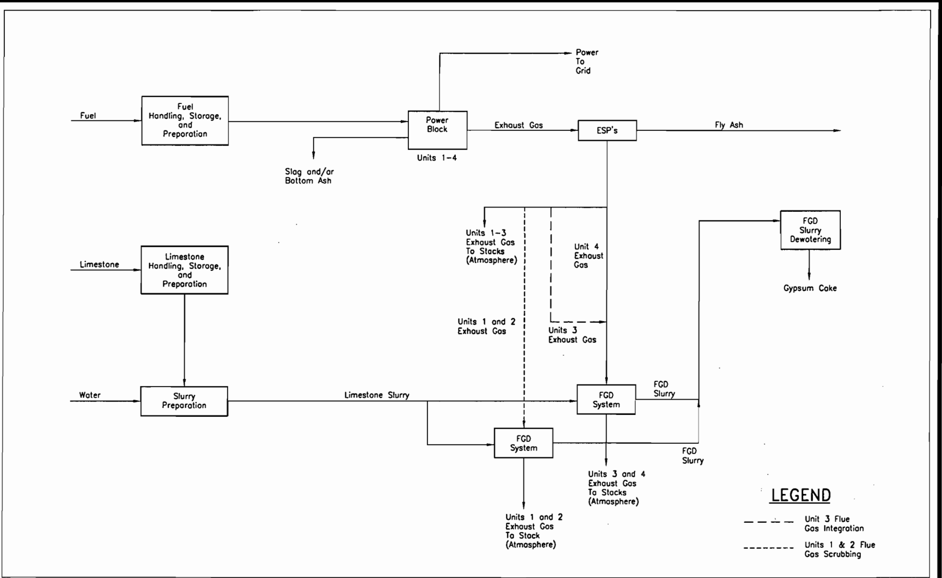
DOCUMENT I.I.E.3.A. OVERALL BOILER PROCESS FLOW DIAGRAM
