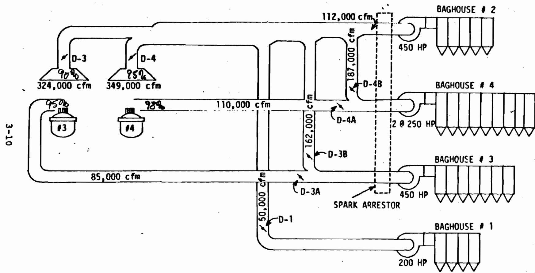
Figure 3-2. Florida Steel, Tampa, damper position and flow rates to baghouses.
