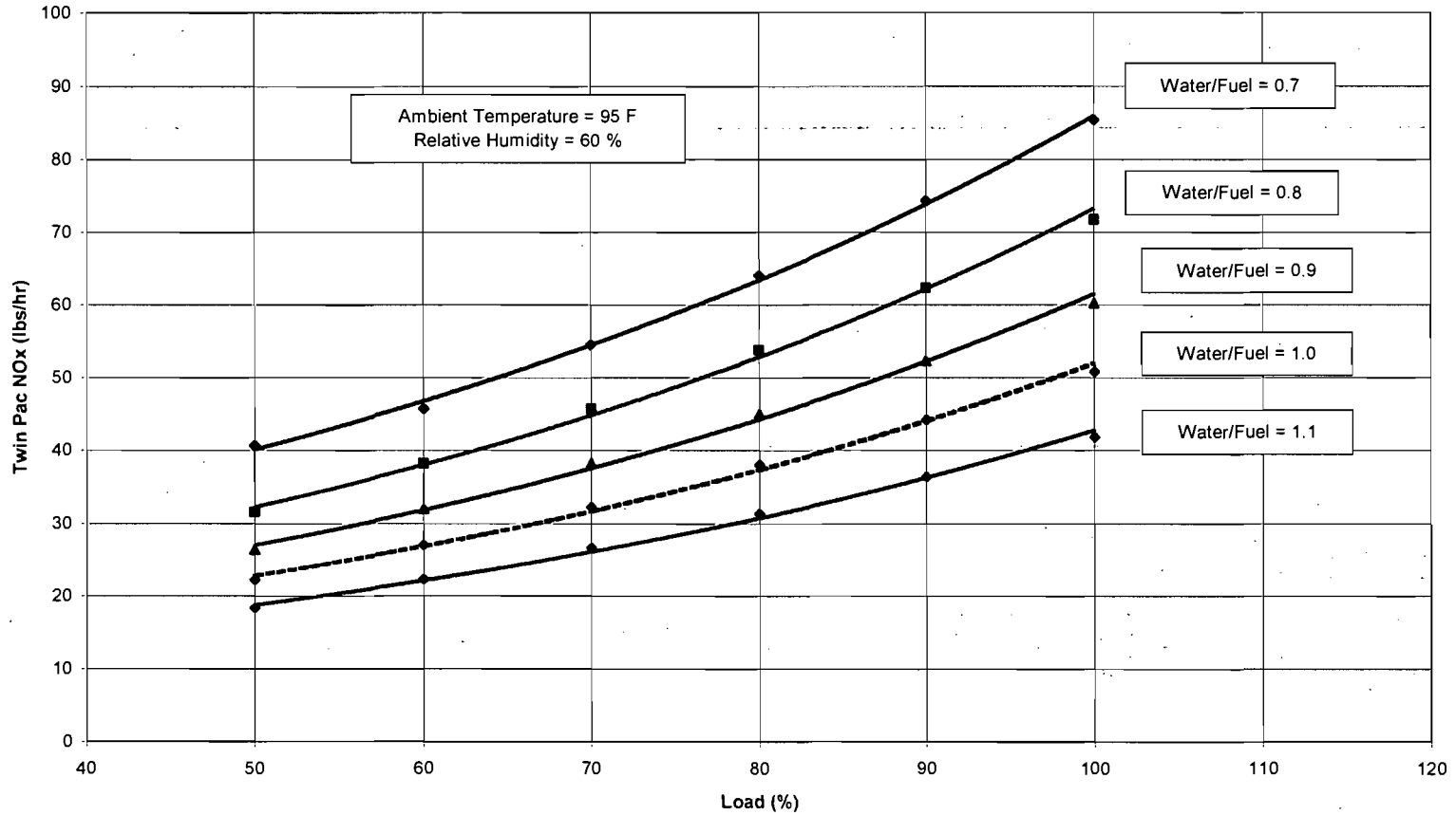
NO x VERSUS LOAD (HOT DAY, AVERAGE HUMIDITY)
