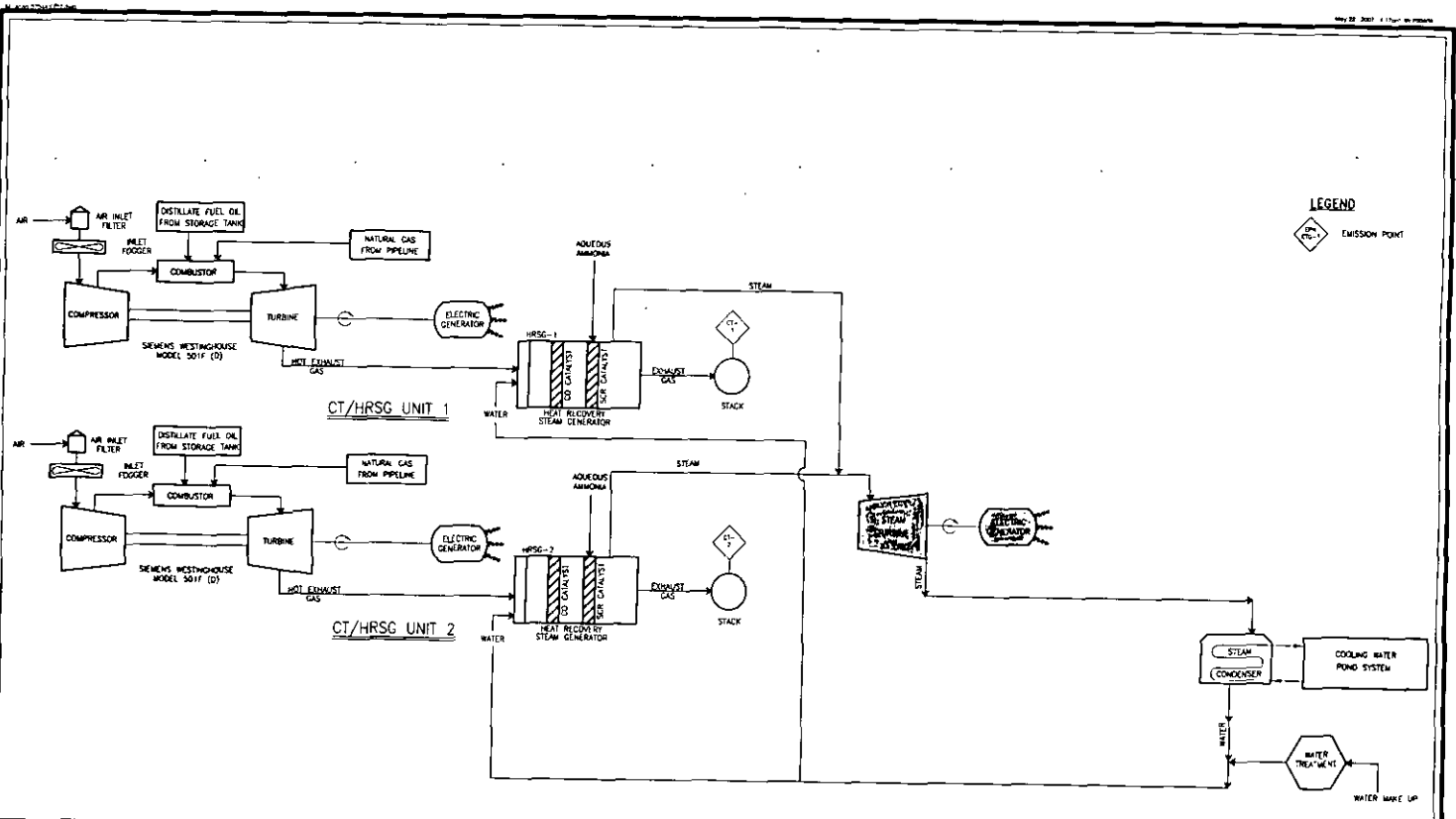
ATTACHMENT 2-A. PAYNE CREEK GENERATING STATION PROCESS FLOW DIAGRAM - COMBINED CYCLE UNITS Source: ECT, 2007
