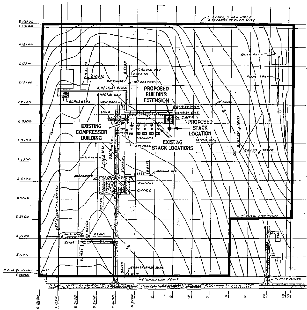
Figure 2-1 PLOT PLAN OF COMPRESSOR STATION NO. 14
