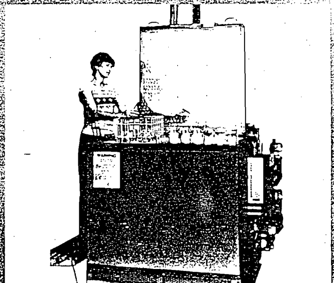
IGG-27 is front loading only and has collection chamber under furnace for maintenance parts.
