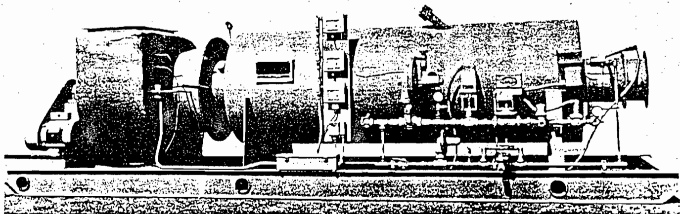
Figure 98. External view of direct-flame afterburner (Gas Processors, Inc., Brea, Calif.).
