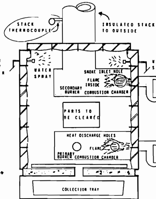
FIGURE 1 SIMPLIFIED OPERATION OF MODEL 166 CONTROLLED PYROLYSIS CLEANING FURNACES
