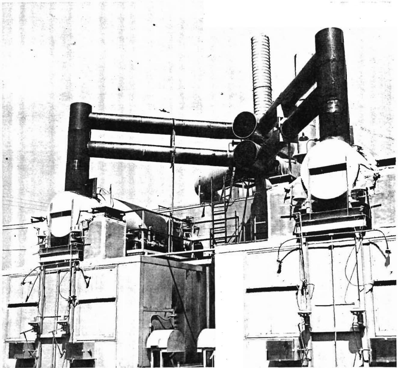
Figure 100. Two direct-flame afterburners controlling venting of organic emissions (American Cyanamid Co., Azusa, Calif.).
