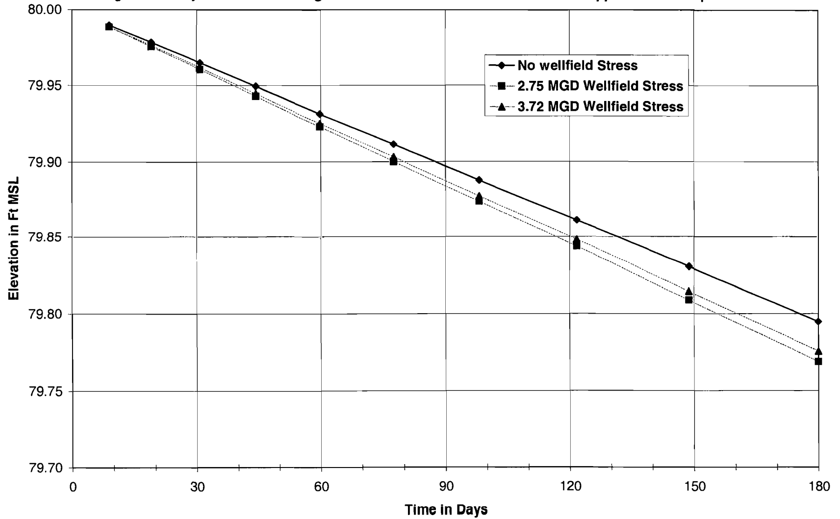
MODFLOW Simulated Changes in Water Table 4000 ft from the Center of the Wellfield. Changes Due only to the downward gradient between the Water Table and the Upper Floridan Aquifer.
