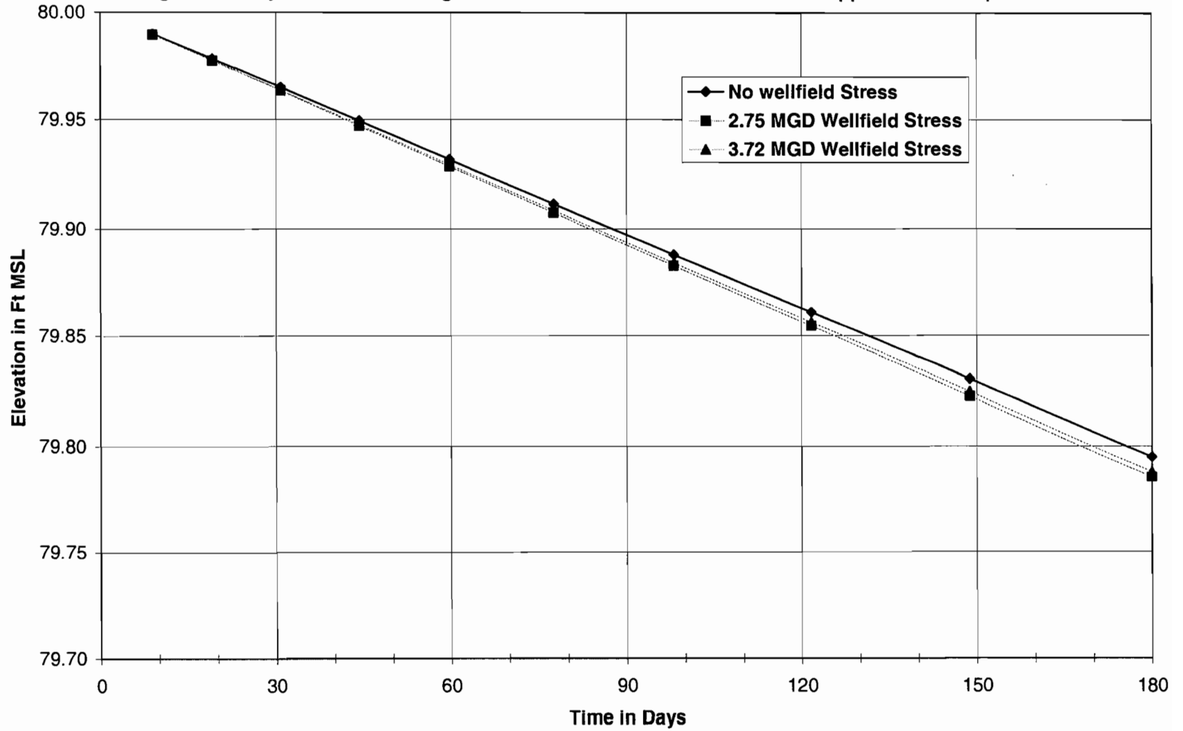
MODFLOW Simulated Changes in Water Table 10,000 ft from the Center of the Wellfield. Changes Due only to the downward gradient between the Water Table and the Upper Floridan Aquifer.
