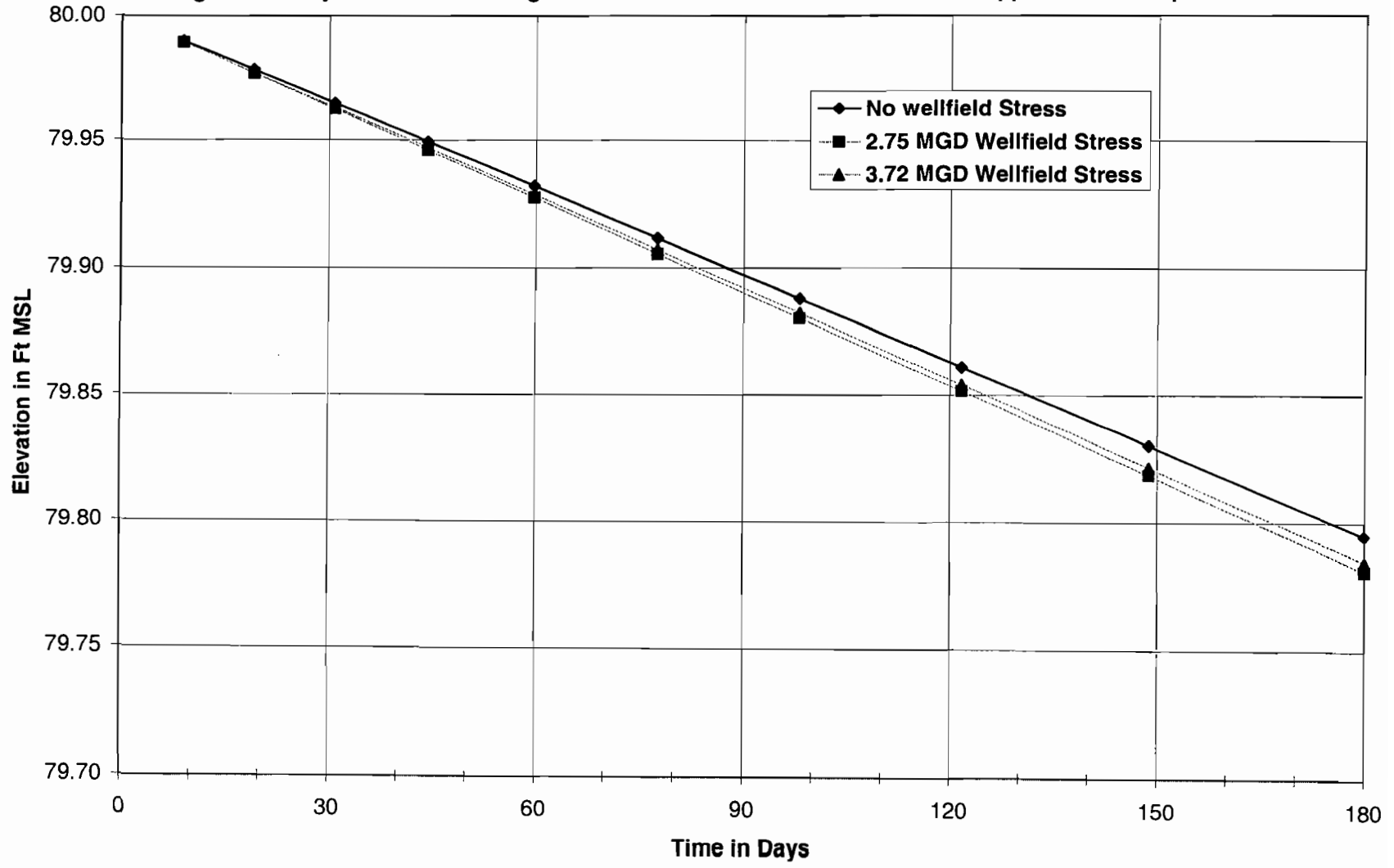
MODFLOW Simulated Changes in Water Table 7500 ft from the Center of the Wellfield. Changes Due only to the downward gradient between the Water Table and the Upper Floridan Aquifer.
