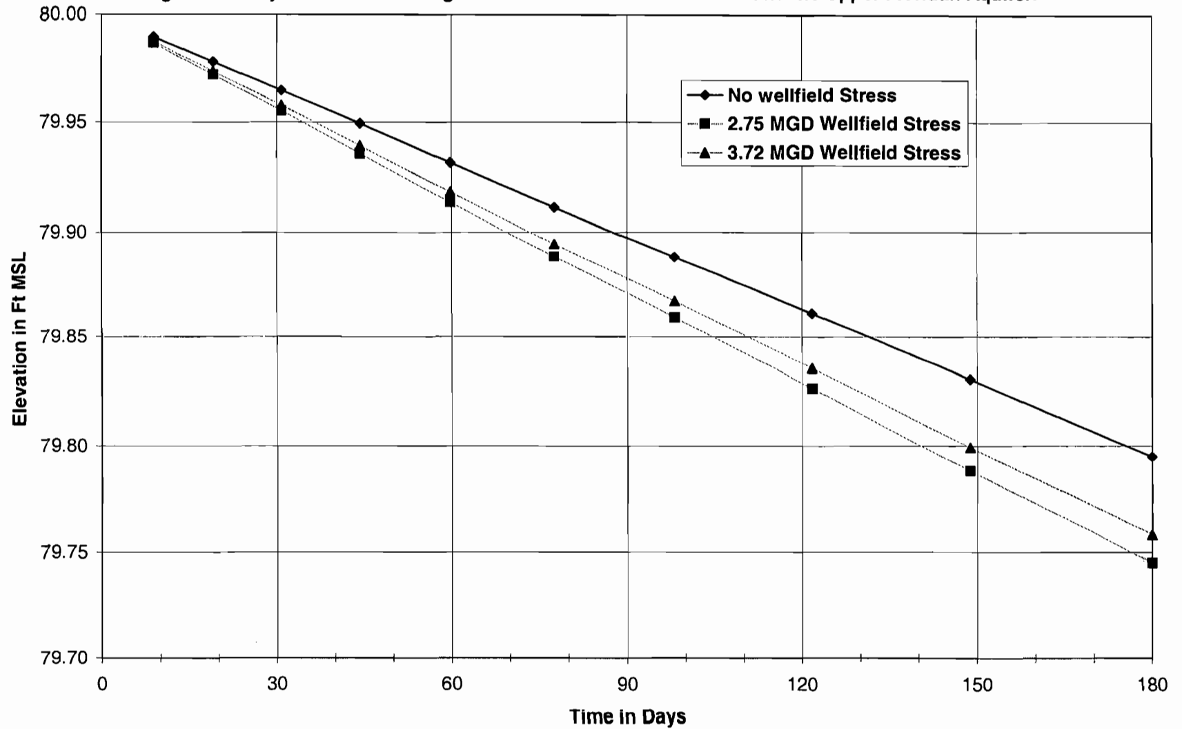
MODFLOW Simulated Changes in Water Table 1000 ft from the Center of the Wellfield. Changes Due only to the downward gradient between the Water Table and the Upper Floridan Aquifer.
