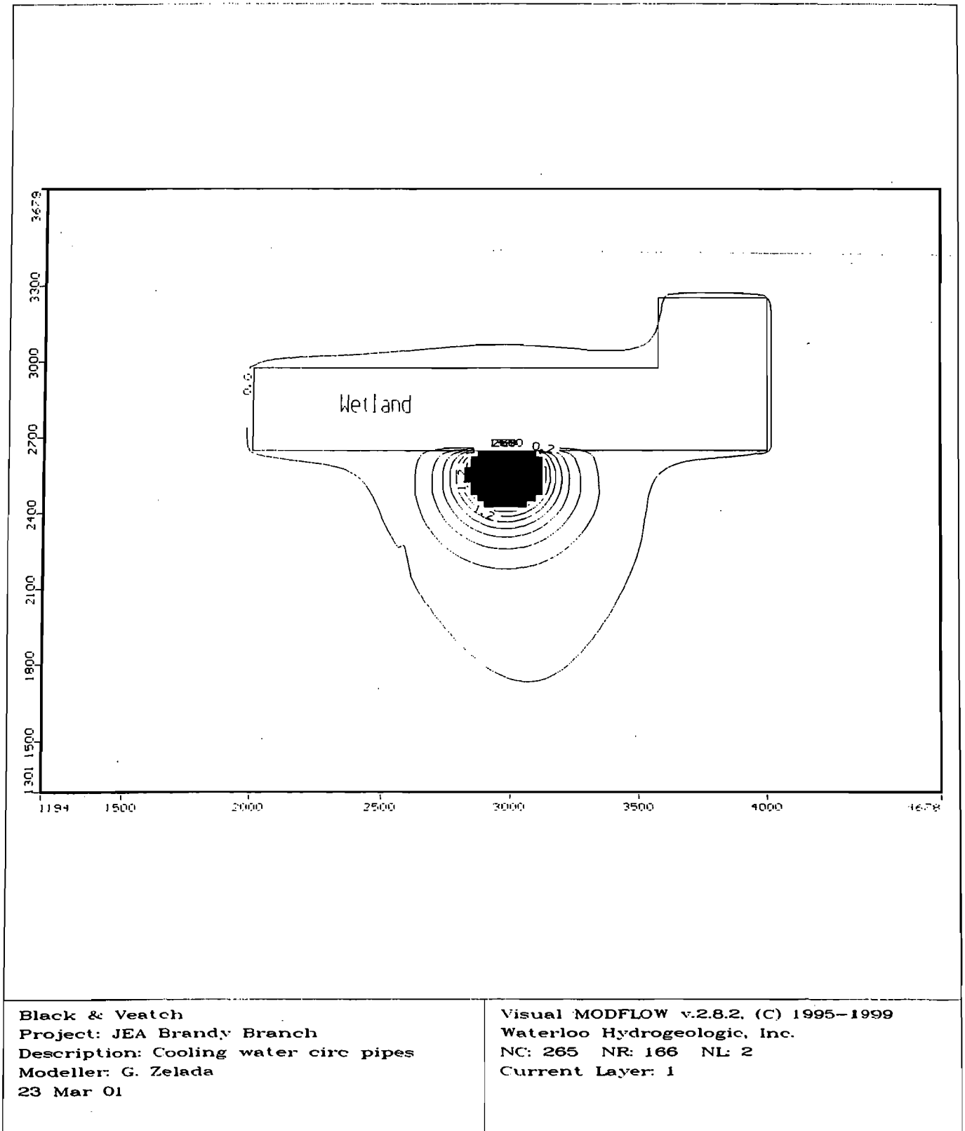
Figure 3: Cooling Water Circulating Pipeline Dewatering
