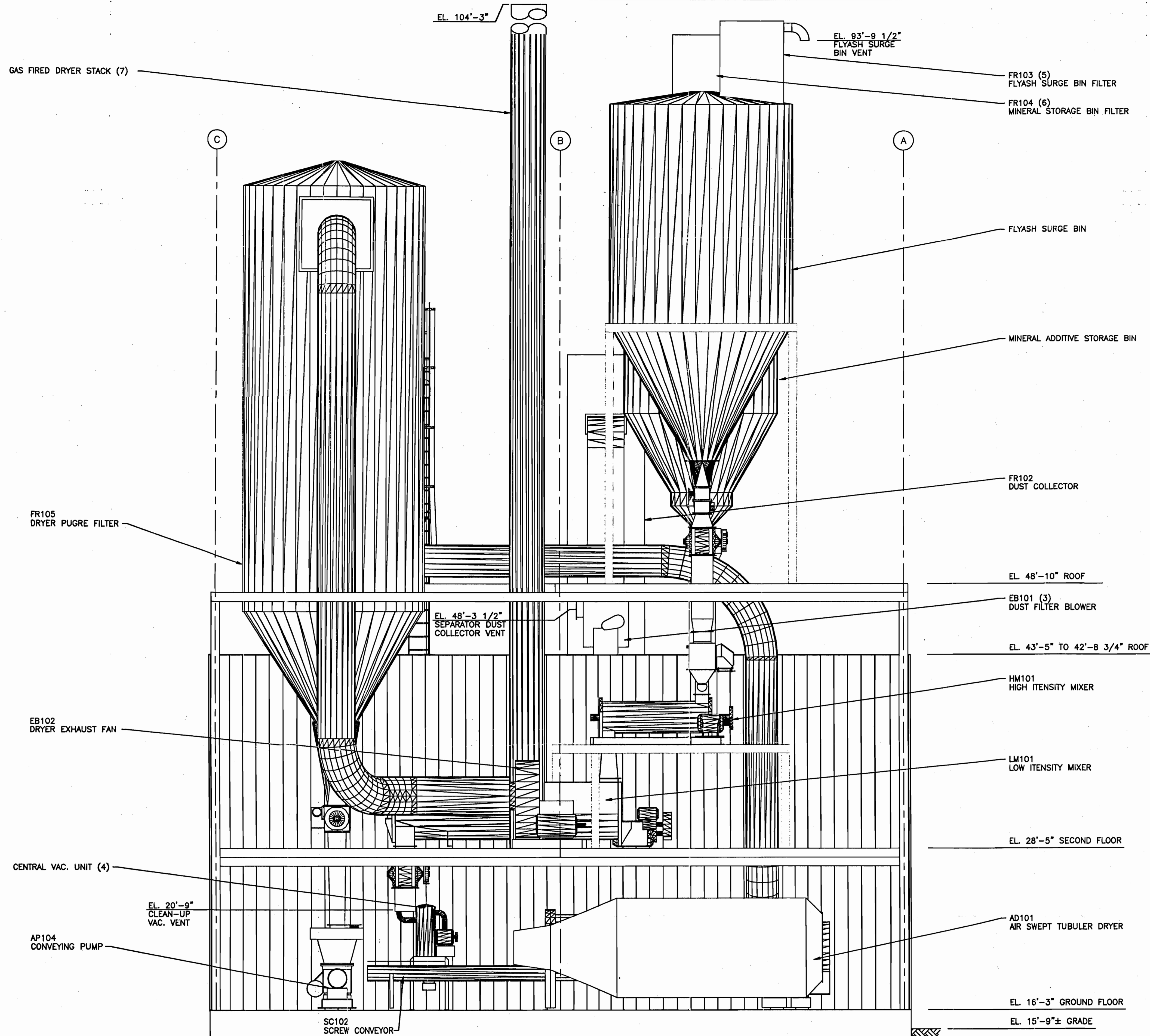
1 EAST ELEVATION (LOOKING WEST) EQS/EQS 1/4"=1'-0"
