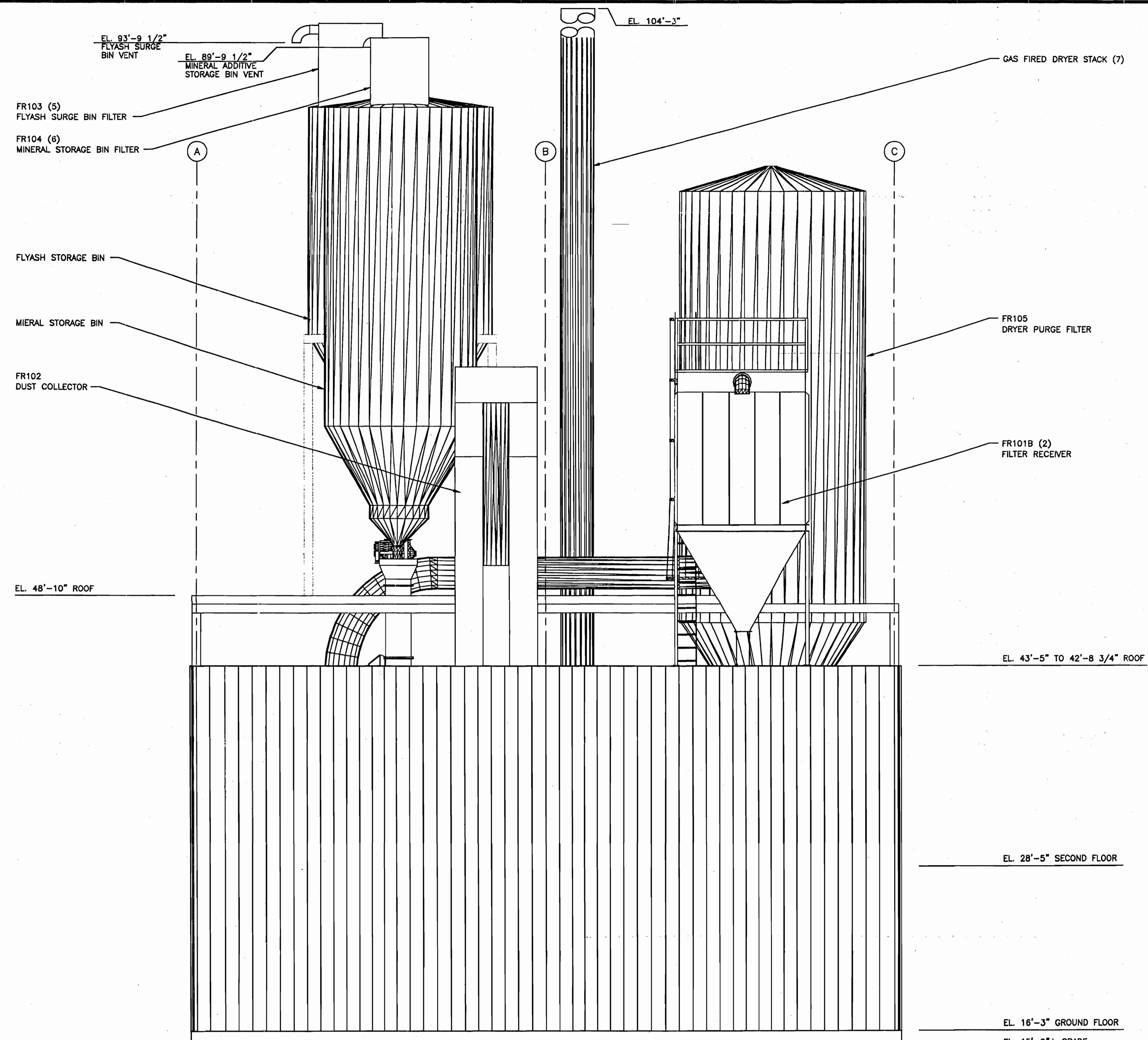
1 WEST ELEVATION (LOOKING EAST) 1/4" = 1'-0"
