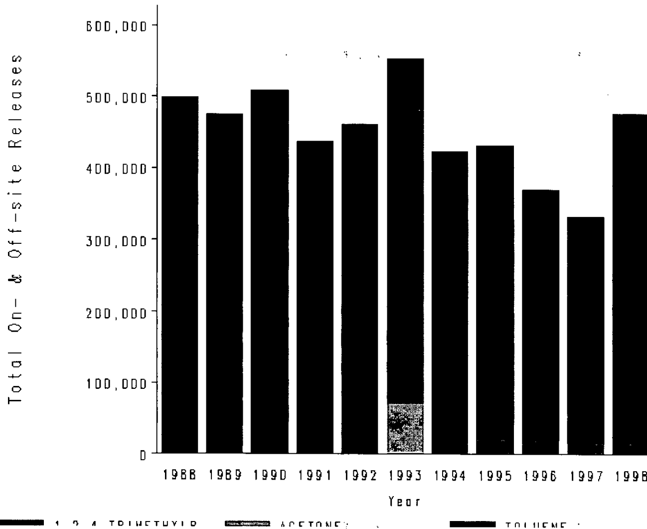
NAILITE INTL. INC. Total On- and Off-site Releases (in pounds), By Chemical
