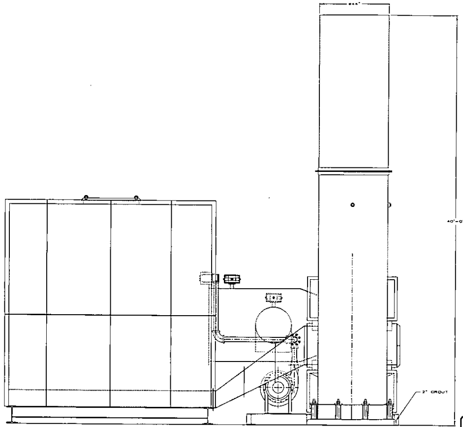
END VIEW
