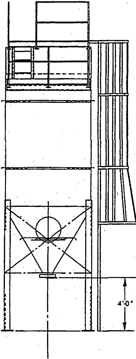
Front elevation.
