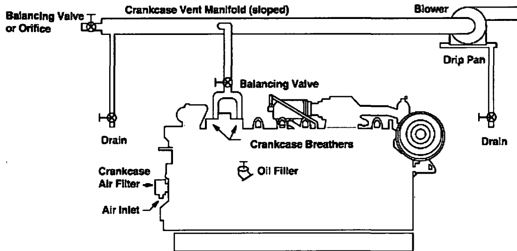
Figure 2. Crankcase Ventilation System
