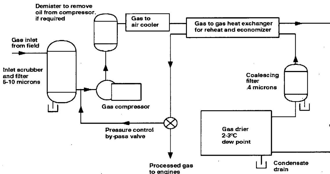
Figure 1. Landfill-Gas-To-Energy – Typical Fuel Treatment System
