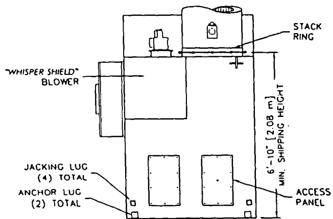
REAR ELEVATION
