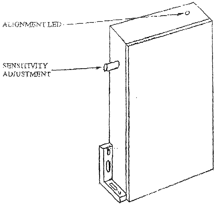
FIGURE 2, OPACITY MONITOR
