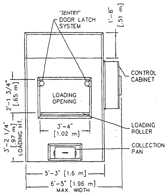
FRONT ELEVATION
