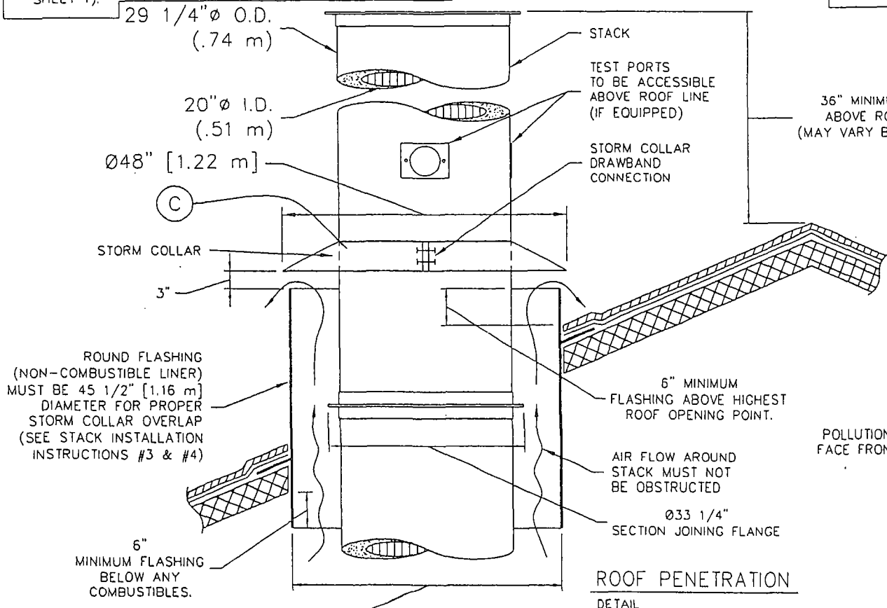
STACK INSTALLATION DETAIL
