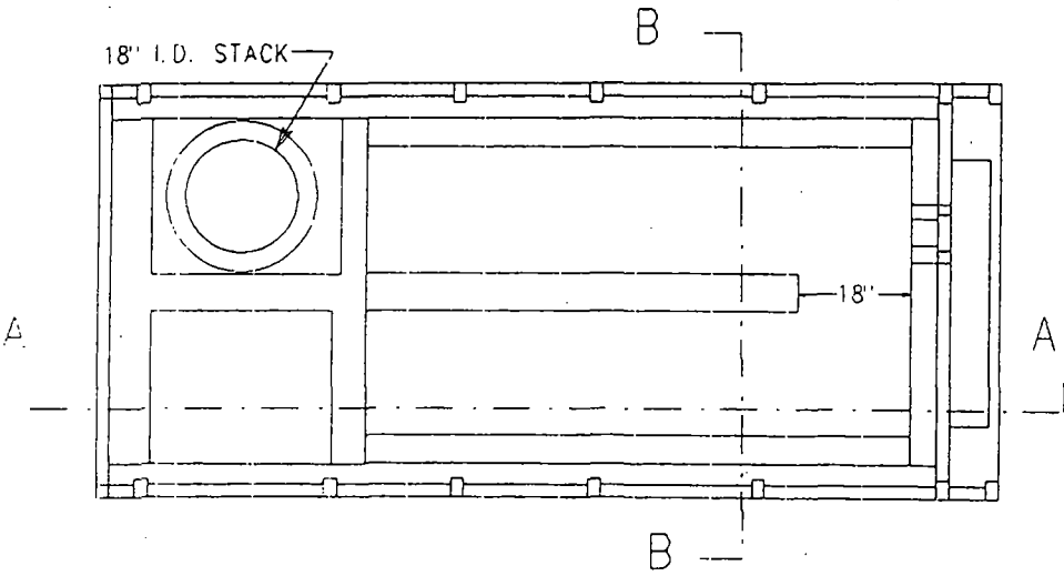
PLAN VIEW THRU CHAMBERS
