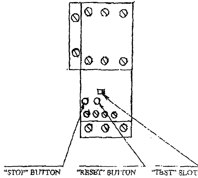
FIGURE 2, OPACITY MONITOR
