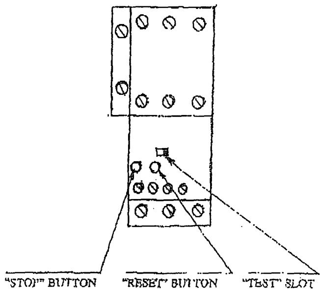
FIGURE 2, OPACITY MONITOR
