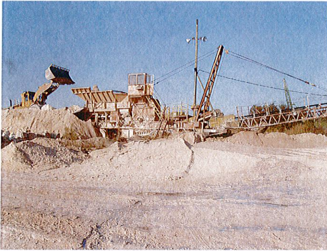
Photo ID No. / Date / Time: Picture 01 03-15-2011 Pioneer Crusher onto Conveyor Belt
