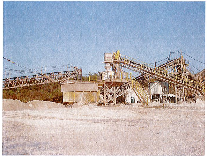
Photo ID No. / Date / Time: Picture 05 03-15-2011 Drop to Screen and Secondary Canica-Jaques Crusher
