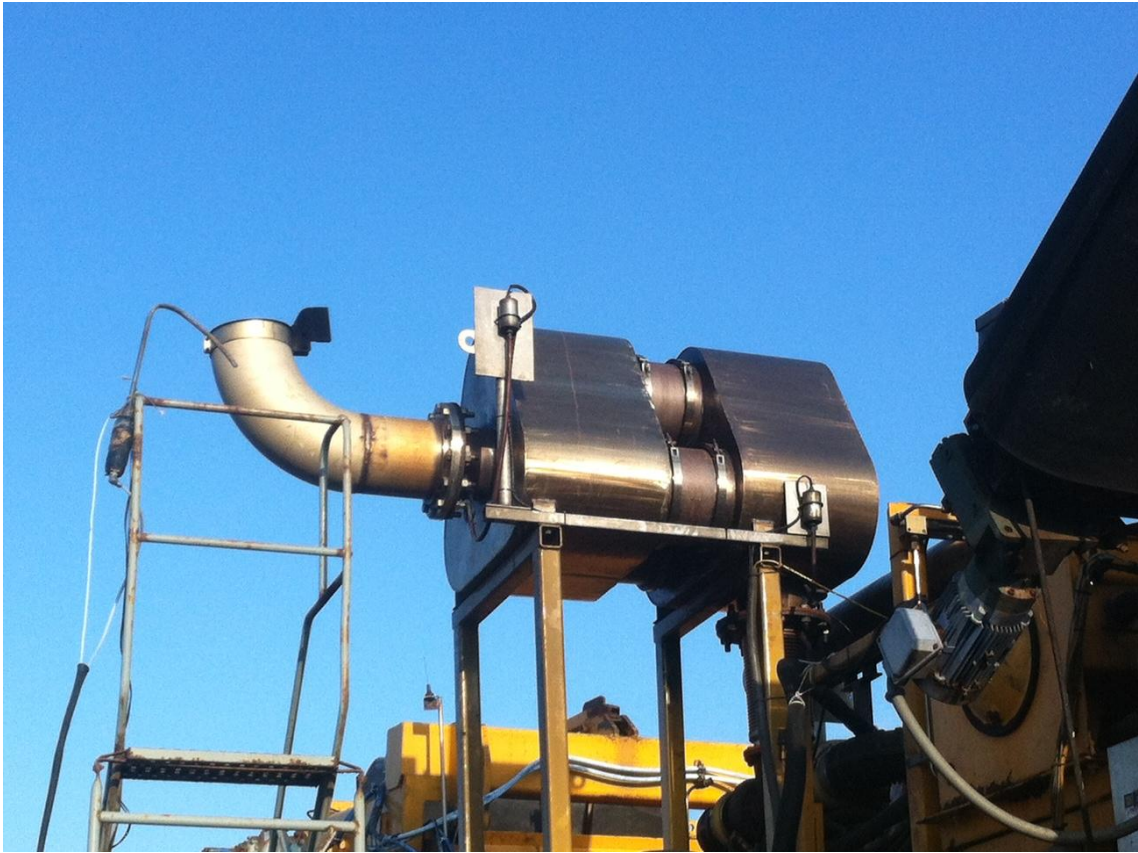
Catalytic Converter Mounted to Woody Waste Diesel Engine 4-3-2013
