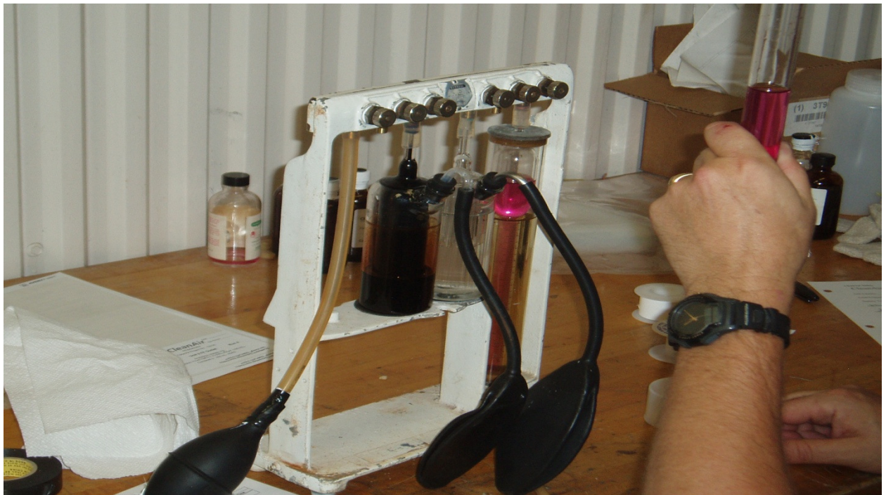
Orsat Analysis from Run 1
